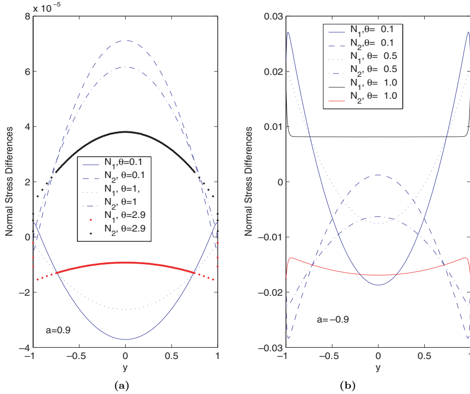
FIG. 6. The normal stress differences N_1 and N_2 in flowing-aligning regimes as functions of y at selected values of \theta with tangentially anchored boundary conditions in weak shear. (a) Rods: a = 0.9 , N = 6 , De = 0.01 , Er = 100 , \alpha = 10 , \mu_1 = 0.01 , \eta = 0.02 . (b) Discs: a = -0.9 , N = 6 , De = 0.01 , Er = 100 , \alpha = 10 , \mu_1 = -0.01 , \eta = 0.02 .
