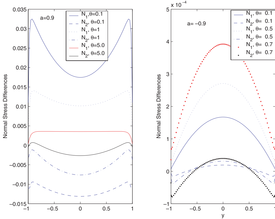
FIG. 9. The normal stress differences N_1 and N_2 as functions of y in flowing-aligning regime at selected values of \theta with normally anchored boundary conditions in weak shear. The parameter values are a = \pm 0.9 , N = 6 , De = 0.01 , Er = 100 , \alpha = 10 , \mu_1 = \pm 0.01 , \mu_2 = 0.02 for rods and discs, respectively.
