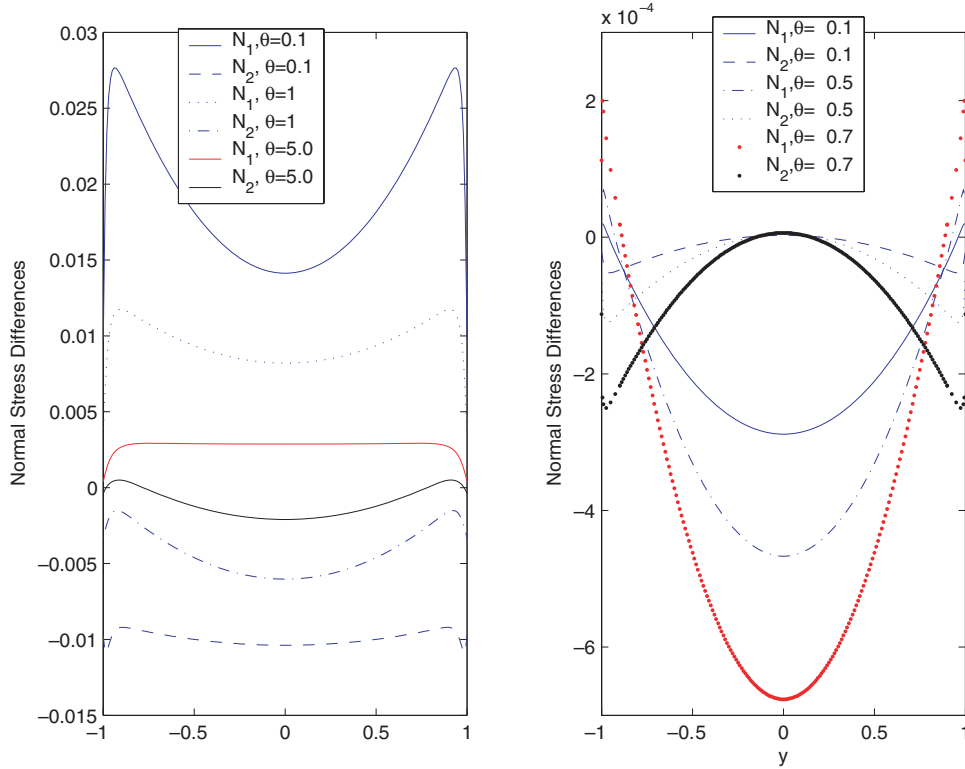
FIG. 8. The normal stress differences N_1 and N_2 as functions of y in tumbling regime at selected values of \theta with normally anchored boundary conditions in weak shear. The parameter values are a = \pm 0.8 , N = 6 , De = 0.01 , Er = 100 , \alpha = 10 , \mu_1 = \pm 0.01 , \mu_2 = 0.02 for rods and discs, respectively.
