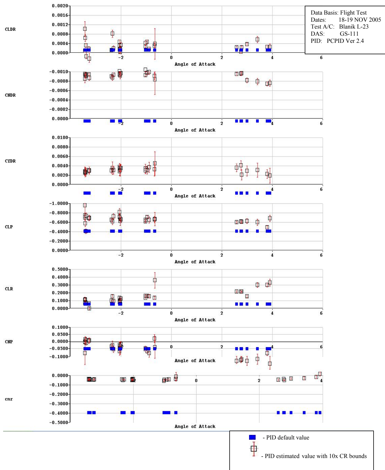
Figure B-6: PID Lateral Directional Derivatives plot (Continued)
