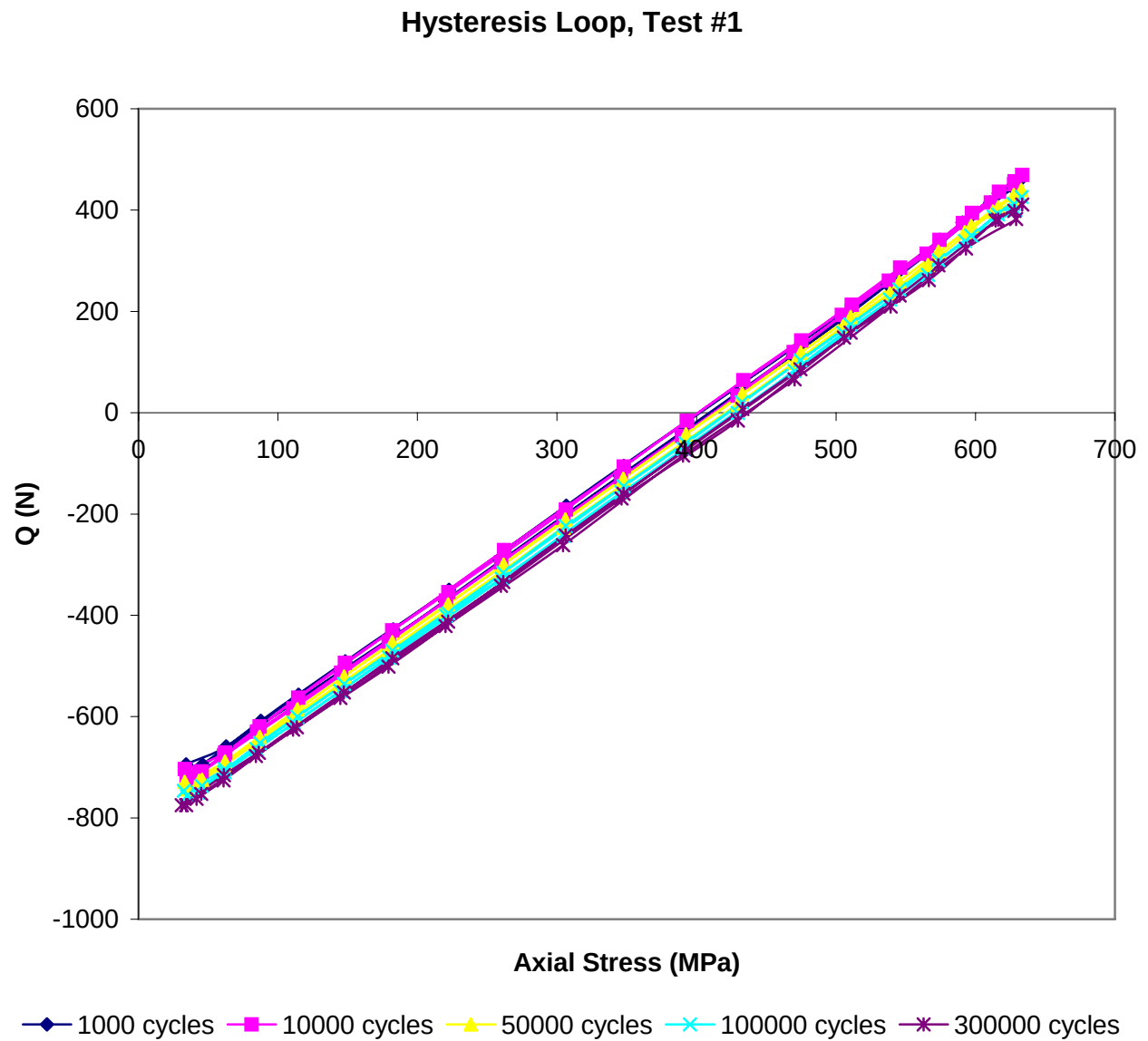
Figure 3.5 Hysteresis Loop
