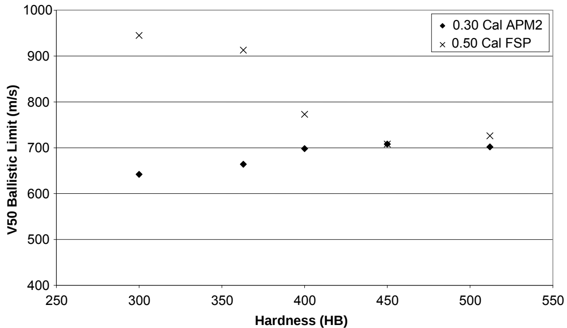
Figure 1. The effect on the V_{50} ballistic limit as the hardness increases for 10 mm Bisalloy plates against 0.30 Cal APM2 and 0.50 Cal FSPs.
