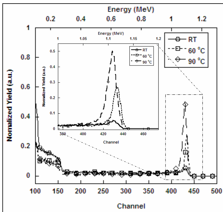
Figure 10. RBS analysis for films comprised of 2k PEG containing 4 weight-percent of 1-DA-3 Au additive after annealing at RT, 60^\circ\text{C} and 90^\circ\text{C} for 24 hr.
