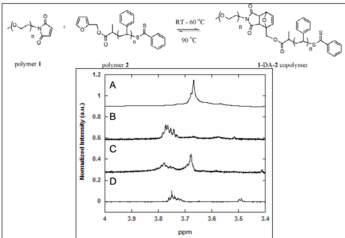
Figure 1. Top: Schematic of model compounds utilized to demonstrate reversible Diels-Alder chemistry. Bottom: ^1\text{H} NMR of polymer 1, polymer 2, and 1-DA-2-copolymer. (a) ^1\text{H} NMR of polymer 1; (b) ^1\text{H} NMR of polymer 2; (c) ^1\text{H} NMR of isolated polymer after heating polymer 1 and polymer 2 at 60\text{ }^\circ\text{C} for 5 days, resulting in 1-DA-2-copolymer; (d) ^1\text{H} NMR of isolated polymer after heating 1-DA-2-copolymer at 90\text{ }^\circ\text{C} for 12 hr, resulting in polymer 2. (Note: A, B, and C are offset by 0.90, 0.59, and 0.27 a.u., respectively, for clarity.)
