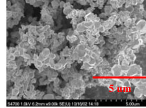
Figure 5. SEM image (SEI) of the starting W powder.
