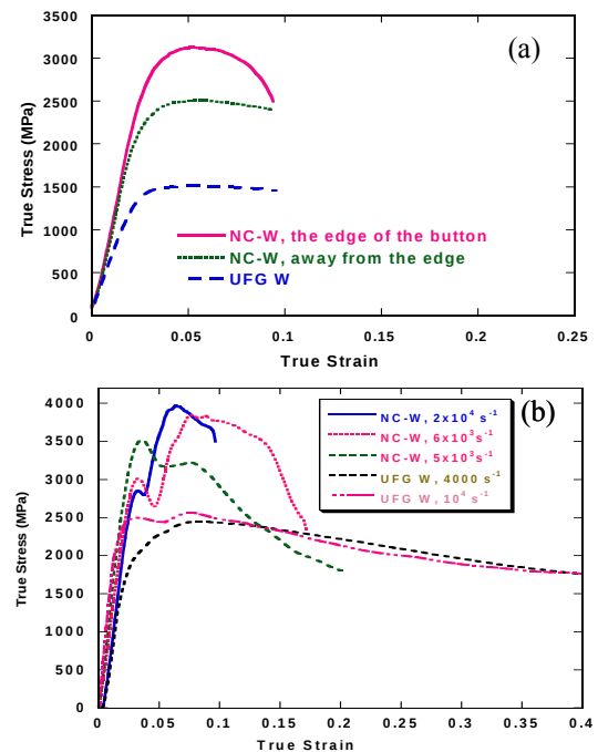
Figure 3. Stress-strain curves of the UFG and NC W under uniaxial compression at quasi-static (a) and dynamic (b) strain rates.
