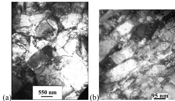
Figure 1. Bright-field TEM images of the (a) UFG-W and (b) NC-W.
