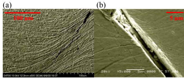
Figure 4. SEM images of (a) UFG W showing severe, localized flow in the shear band; and (b) NC W showing extreme localization and separation.
