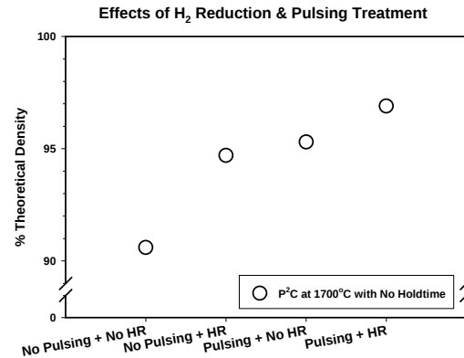
Figure 6. W sample density as a function of \text{H}_2 reduction and current pulsing.
