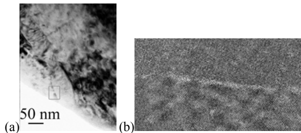
Figure 2. Bright field TEM image of the NC W structure is shown in (a); high-resolution TEM image of the boxed region is shown in (b).
