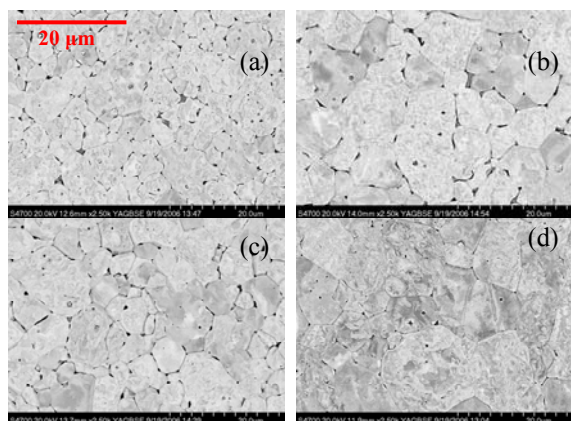
Figure 7. SEM images the W samples: (a) no treatment; (b) H 2 reduction only; (c) pulsing only; and (d) H 2 reduction and pulsing; same magnification in all images.
