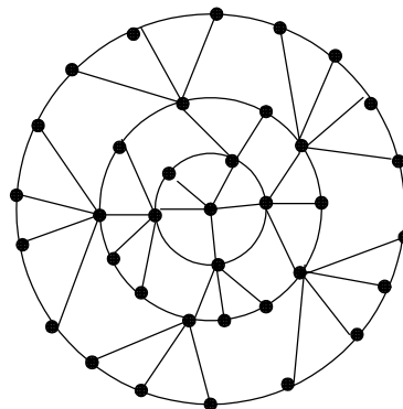
Figure 2-2: MPR Tree.
