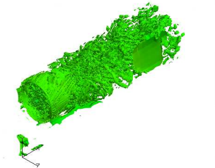
(b) Instantaneous axial vorticity iso-surface.
