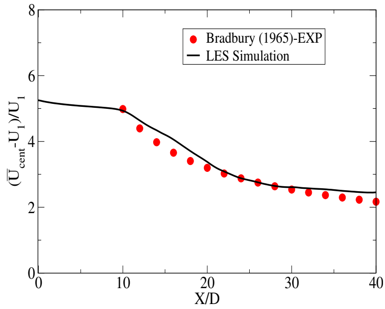
Figure 82: Mean centerline axial velocity (validation case)
