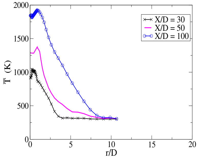
Figure 66: Mean radial soot temperature profiles
