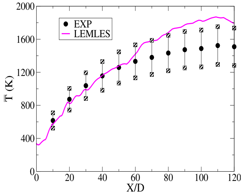
Figure 65: Mean axial temperature with error bars superimposed
