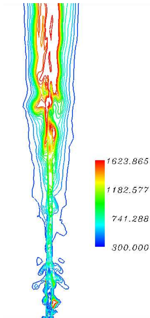
(b) Instantaneous temperature contours.
