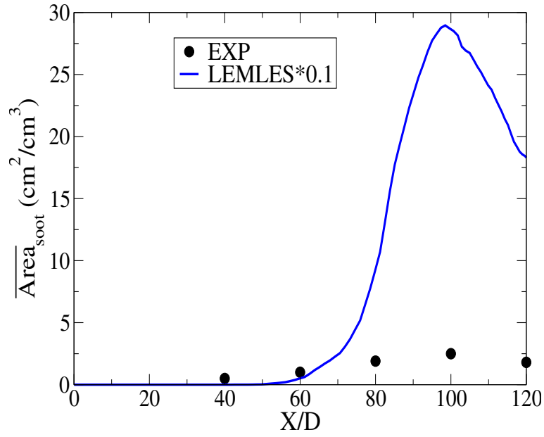
Figure 75: Mean axial average soot surface area per unit mixture volume
