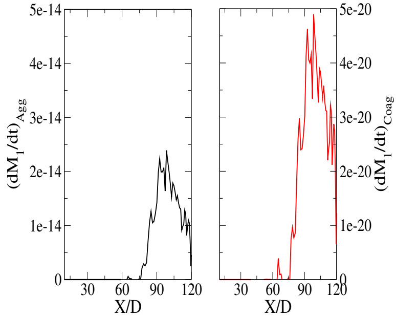
Figure 69: Comparison of the first moment rate with aggregation (left) and coagulation (right)
