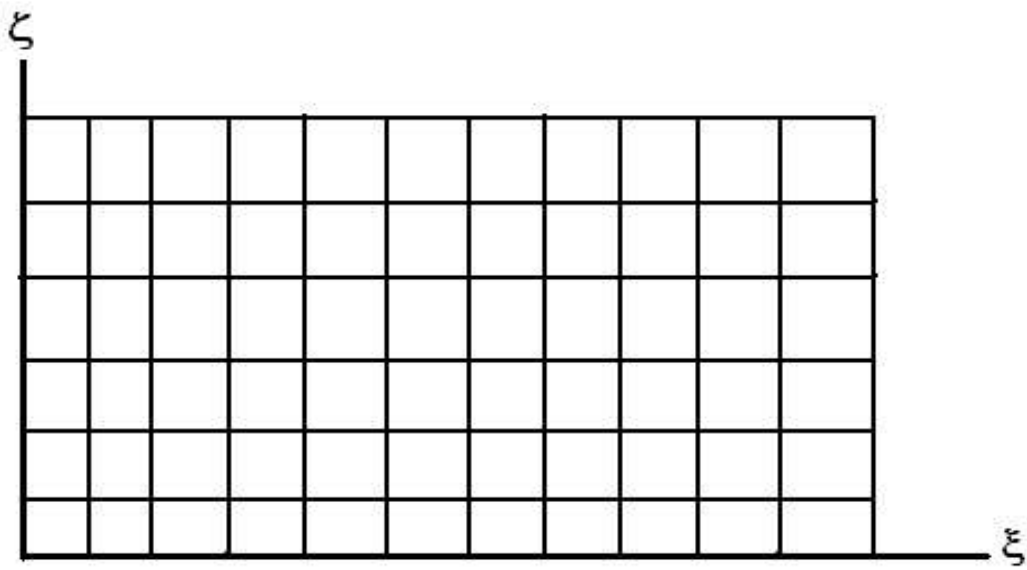
Figure 11: The corresponding computational domain
