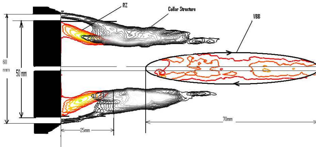
Figure 45: Flow field structure for the cold flow test case
