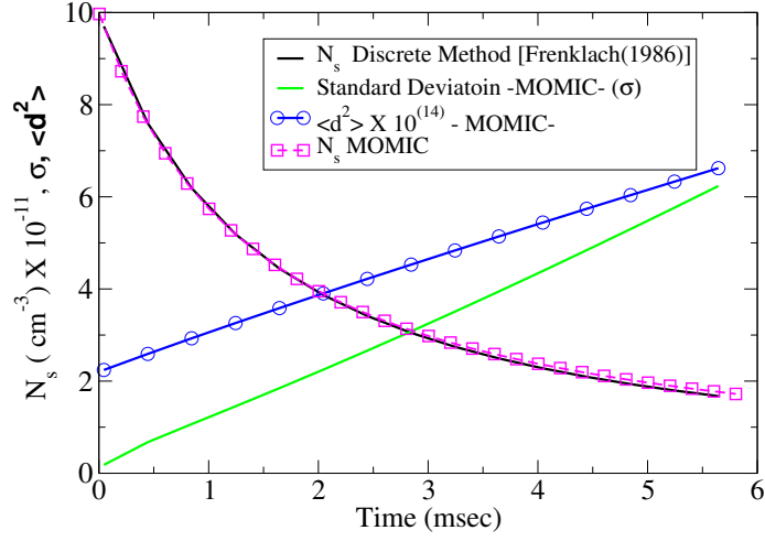
(a) Test case A. (coagulation only)
