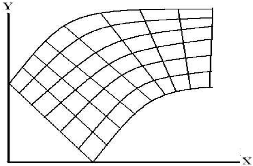
Figure 10: A two dimensional physical domain.
