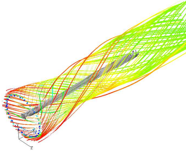
Figure 53: The mean velocity streamlines
