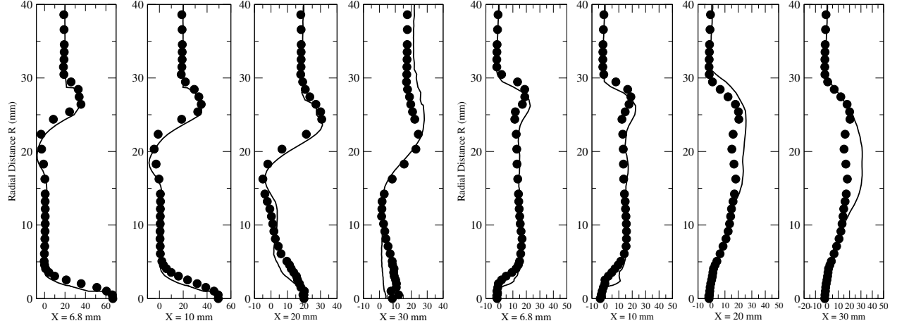
(a) \overline{U_x} (m/sec).
