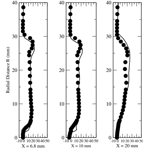
(b) \overline{W}_\theta (m/sec).
