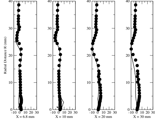
(c) \overline{V_r} (m/sec).
