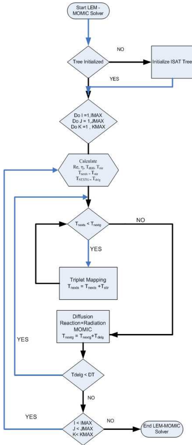
Figure 7: Flow chart for the LEM solver
