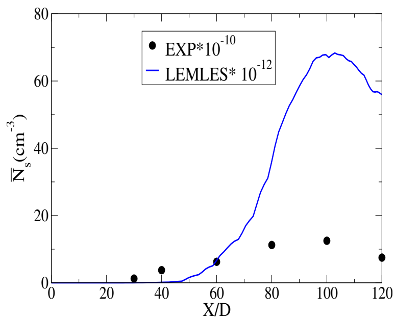
Figure 73: Mean axial number density
