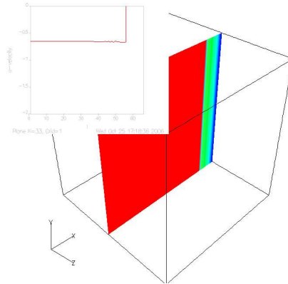
(e) Pressure wave t = t4 .
