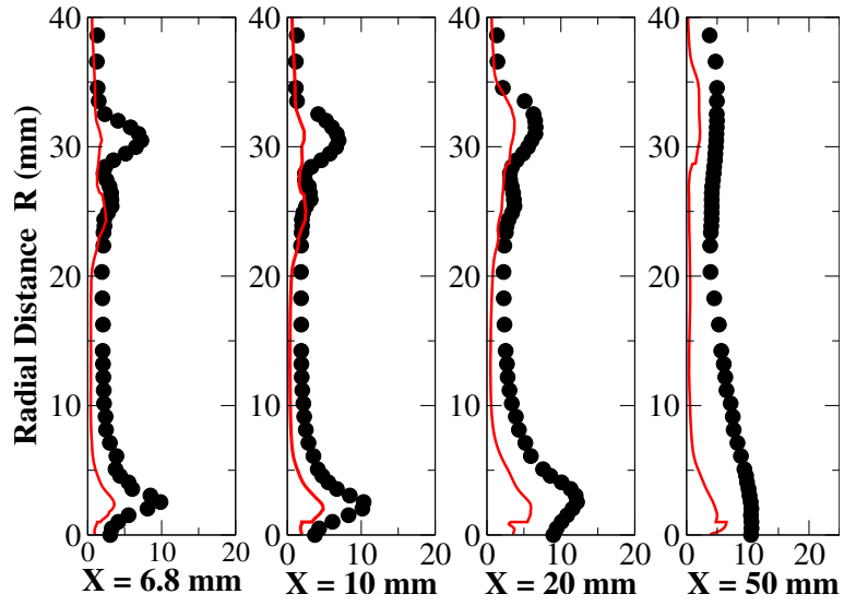
(b) Azimuthal RMS, W_{\theta,rms} .
