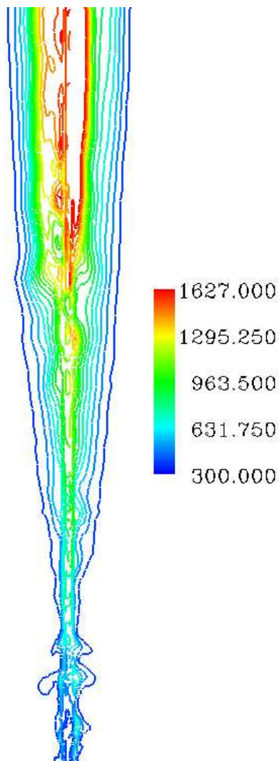
(a) Average temperature contours, \overline{T} .
