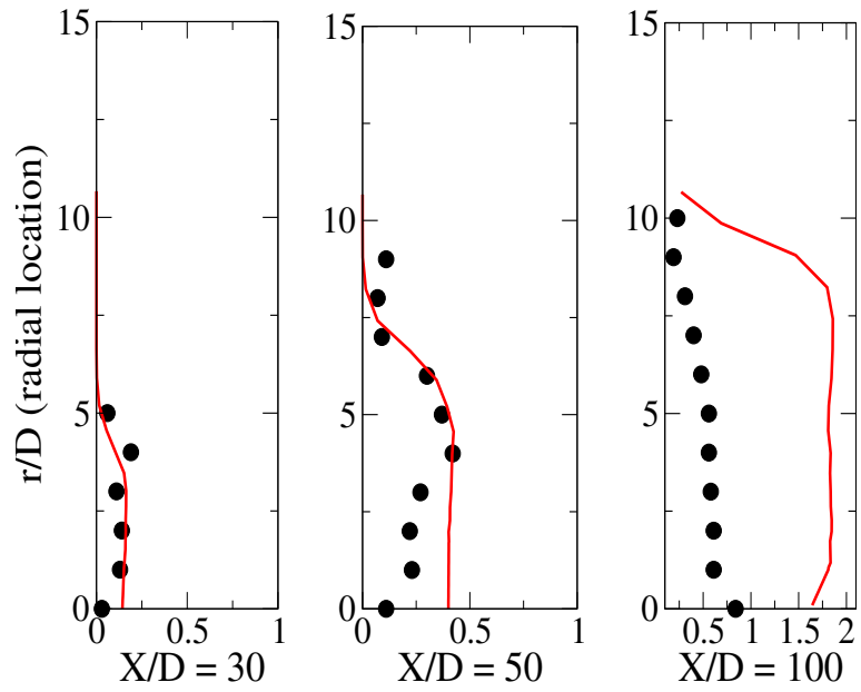
Figure 70: Mean radial soot volume fraction profiles
