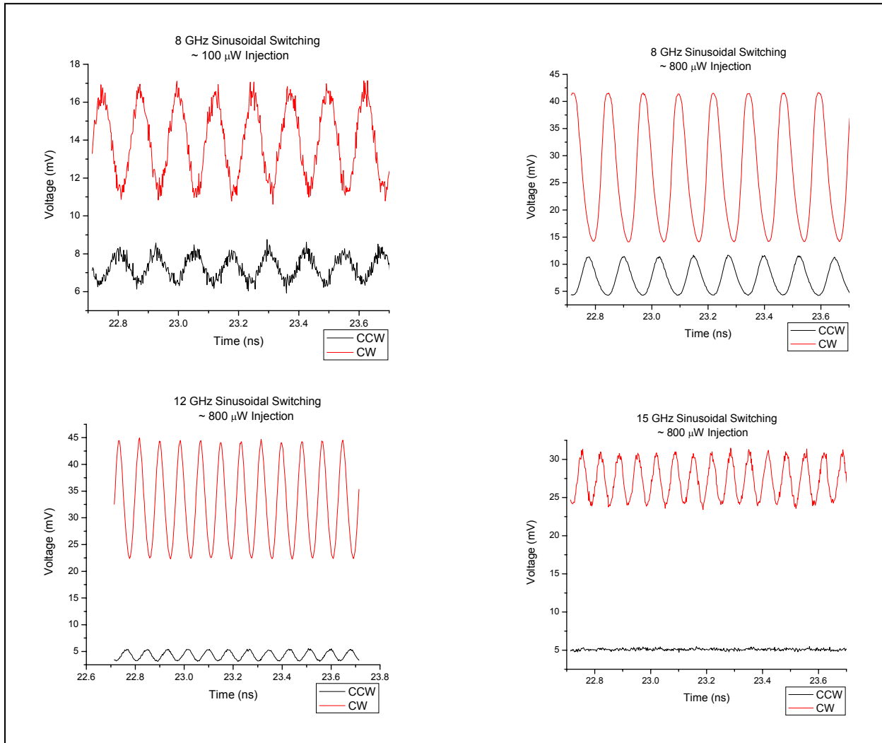
Figure 30. Eight GHz sinusoidal modulation for 100 \mu W and 800 \mu W injected powers with the extinction ratio reducing to < 3 dB at 12 GHz and virtually no response at 15 GHz at 800 \mu W injected powers.
