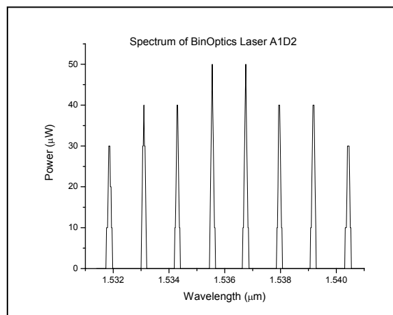
Figure 11. Resonant wavelengths of the A1D2 ring laser.
