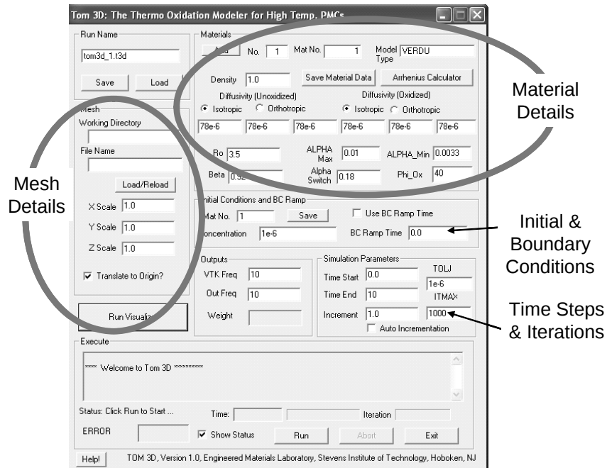
Fig. 14. User input interface for TOM-3D
