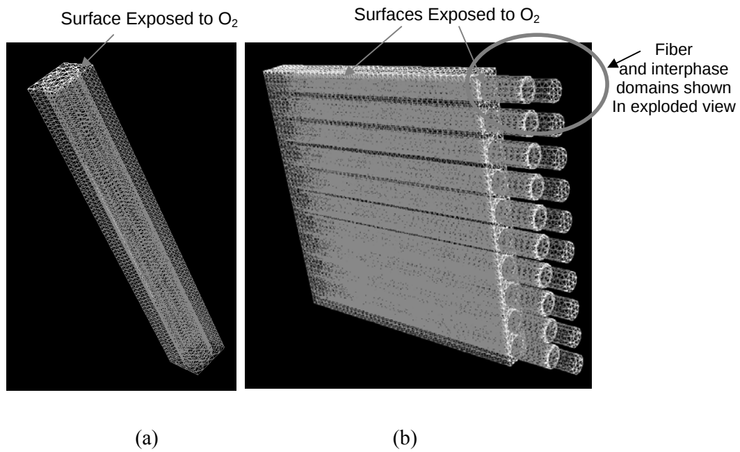
Fig. 15. Representative volume elements used for the analyses
