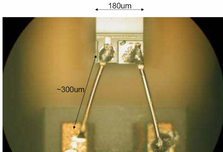
Figure 3 Photograph of the wire-bonded EAM.
