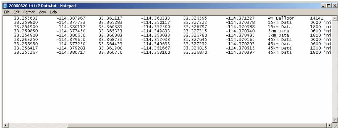
Figure 23. Sample text file record of CARP and OP calculations from the JPADS-MP captured by the Screen OCR program.
