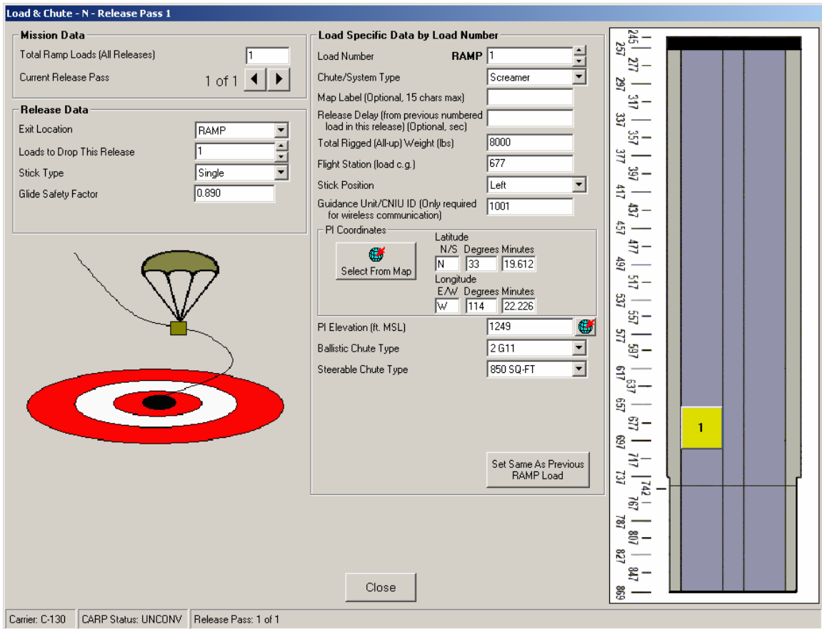
Figure 48. Load & Chute GUI
