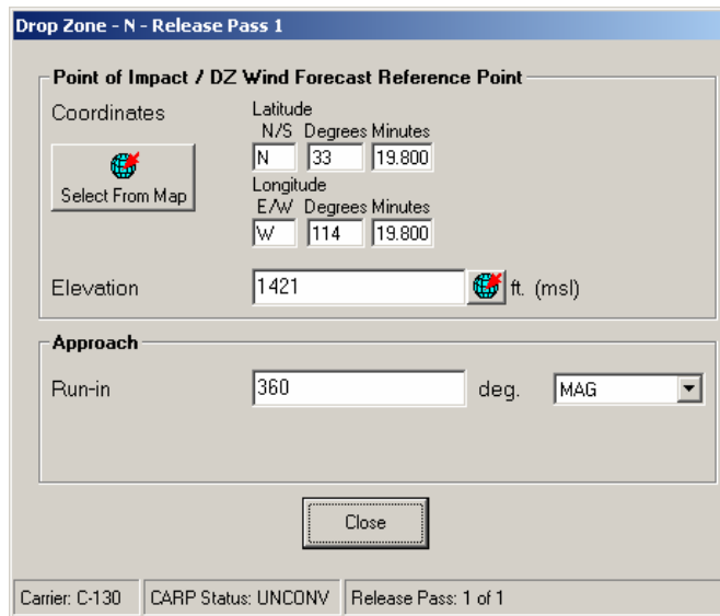
Figure 46. Drop Zone GUI
