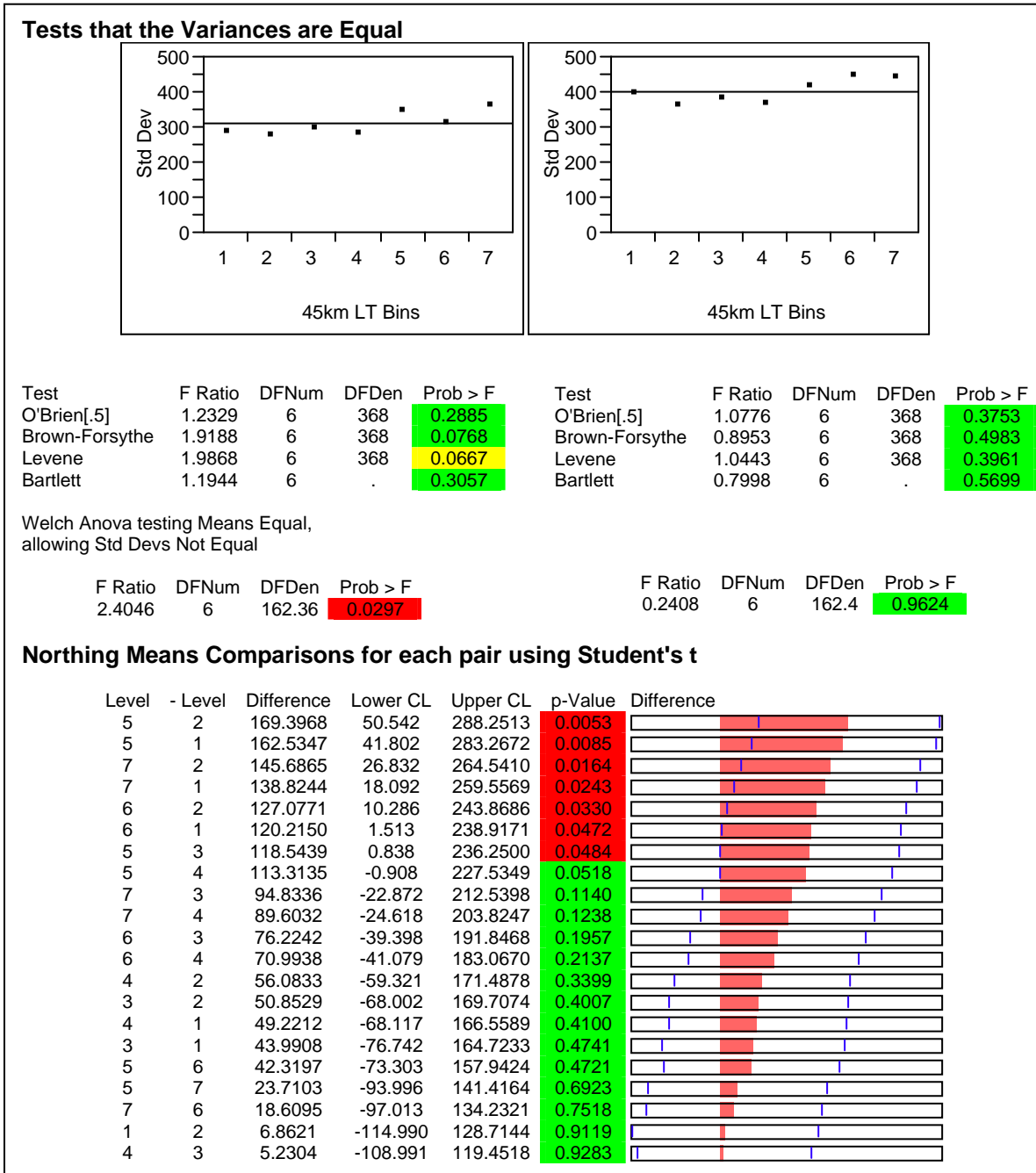
Figure 40. JMP 6 Oneway Layout Analysis of 45km Resolution data, Part 2
