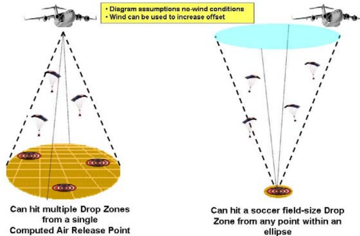
Figure 5. JPADS Guided Parachute drop capabilities (6)
