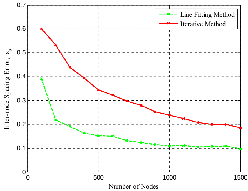
Figure 27. Average Inter-node Spacing Error \varepsilon_s for 300 MHz and 7 Linear Nodes Antenna Array for 1000 Monte Carlo Runs as a Function of the Number of Nodes in the Sensor Field
