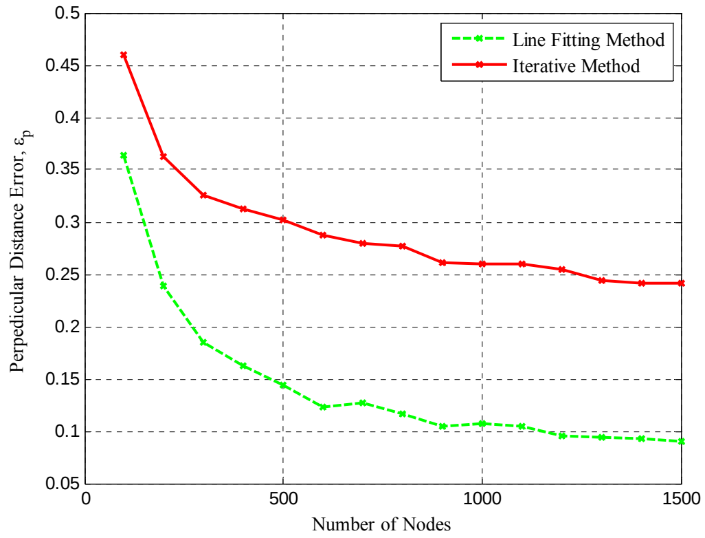
Figure 32. Average Perpendicular Distance Error \varepsilon_p for 300 MHz and 9 Nodes Linear Antenna Array for 1000 Monte Carlo Runs as a Function of the Number of Nodes in the Sensor Field
