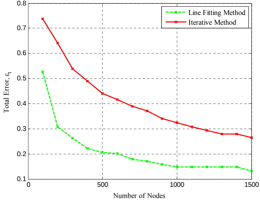
Figure 28. Average Total Error \varepsilon_t for 300 MHz and 7 Nodes Antenna Array for 1000 Monte Carlo Runs as a Function of the Number of Nodes in the Sensor Field
