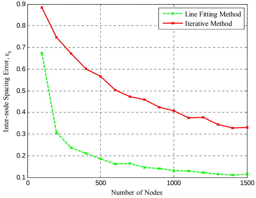
Figure 33. Average Inter-node Spacing Error \epsilon_s for 300 MHz and 9 Nodes Linear Antenna Array for 1000 Monte Carlo Runs as a Function of the Number of Nodes in the Sensor Field
