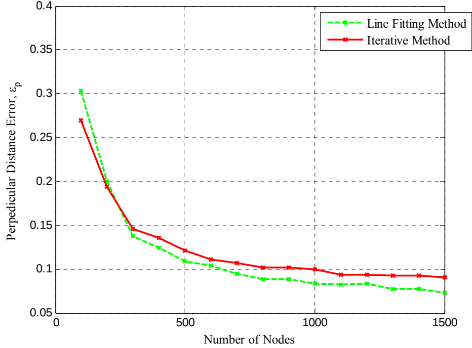
Figure 36. Average Perpendicular Distance Error \epsilon_p for 900 MHz and 7 Nodes Linear Antenna Array for 1000 Monte Carlo Runs as a Function of the Number of Nodes in the Sensor Field
