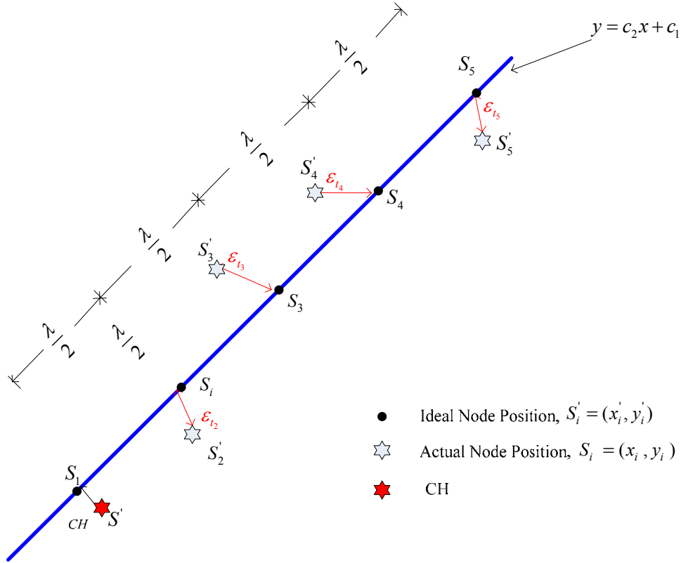
Figure 22. Total Error Calculation
