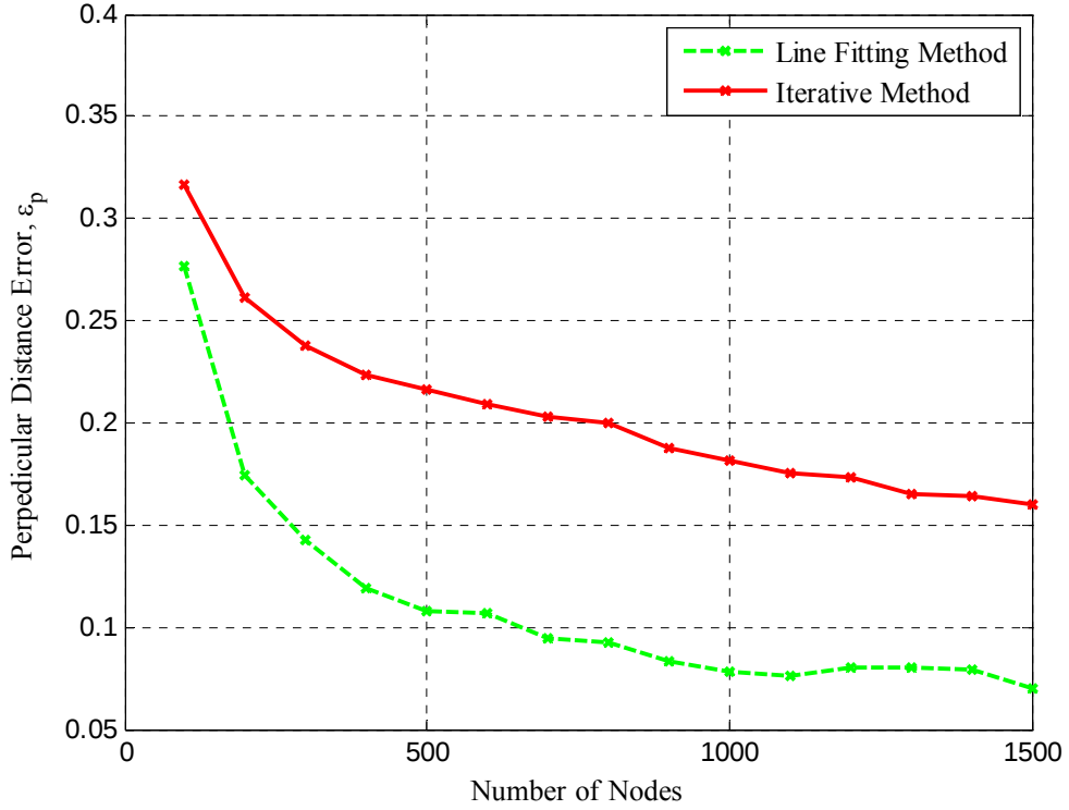
Figure 26. Average Perpendicular Distance Error \epsilon_p for 300 MHz and 7 Nodes Linear Antenna Array for 1000 Monte Carlo Runs as a Function of the Number of Nodes in the Sensor Field
