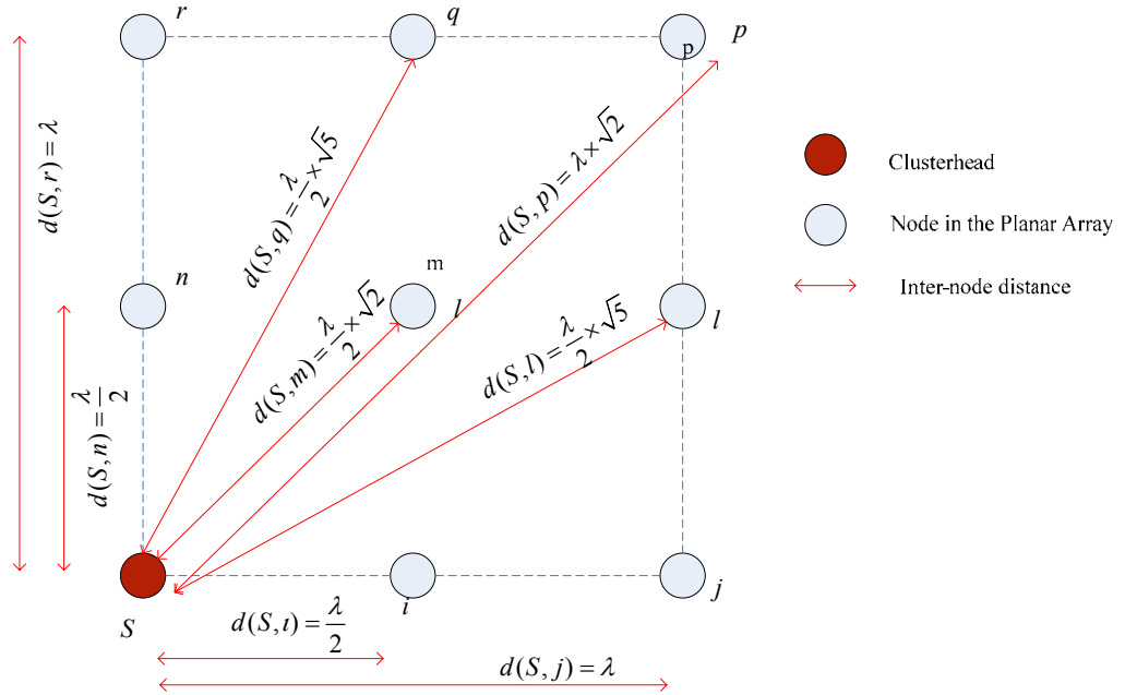
Figure 16. Node Distances from the CH in a 3 \times 3 Array
