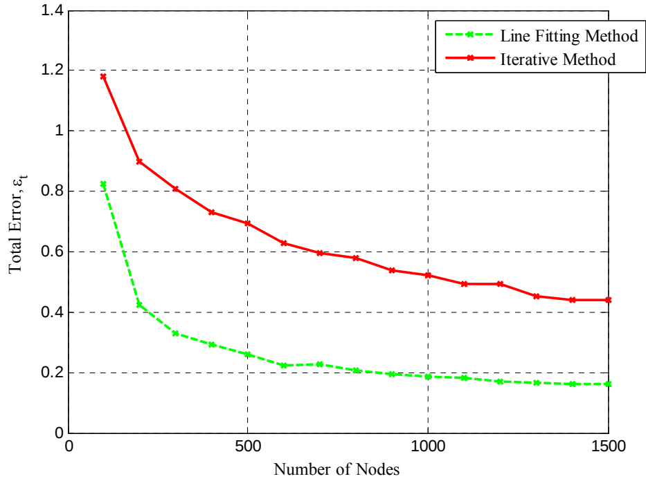
Figure 34. Average Total Error \epsilon_t for 300 MHz and 9 Nodes Linear Antenna Array for 1000 Monte Carlo Runs as a Function of the Number of Nodes in the Sensor Field
