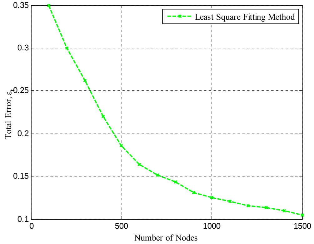
Figure 47. Average Total Error \varepsilon_t for 300 MHz and 4 \times 4 Nodes Planar Antenna Array for 100 Monte Carlo Runs as a Function of the Number of Nodes in the Sensor Field
