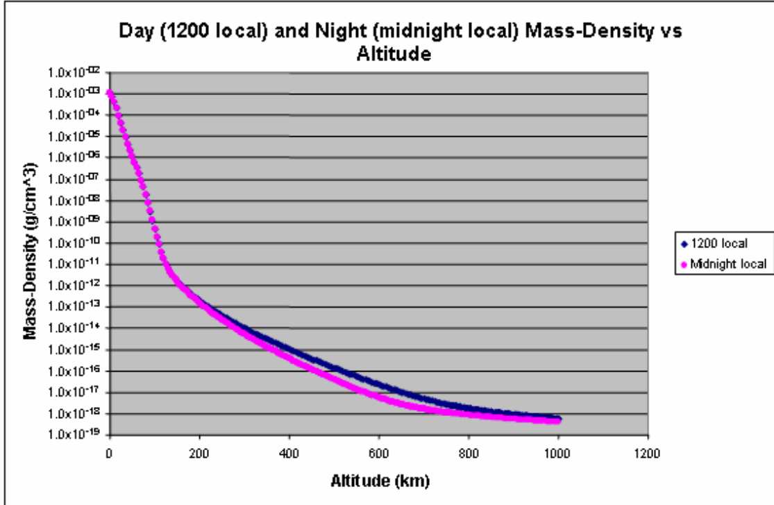
Figure 4.2.1: The semi-log plot of the mass density vs. altitude is shown for values from the MSIS code for 6 August 1965. The purple (lowest dipping curve) represents the midnight density and the blue represents the midday density. The density can vary up to an order of magnitude between day and night. For the computer simulation, an average of the day and night densities is used.
