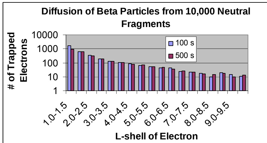
Figure 7.4.3.1: The spread of the electrons is shown resulting from a release of 10,000 neutral fission fragments at an L-shell value of 1.176. The neutral fragments move away from the injection location and some beta decay before penetrating the earth's atmosphere or traveling off into space.
