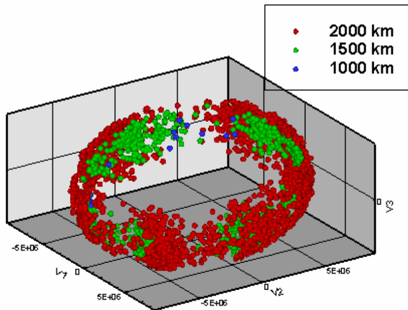
Figure 7.3.3: The location of the electrons 1,000 s after the release of the ions at three of the four different altitudes. There were only two electrons remaining from the release of fission fragments at 500 km. Like the ions, the electrons from the 1,500-km and 2,000-km release altitude are dispersed around the earth and not experiencing major losses at the SAA.
