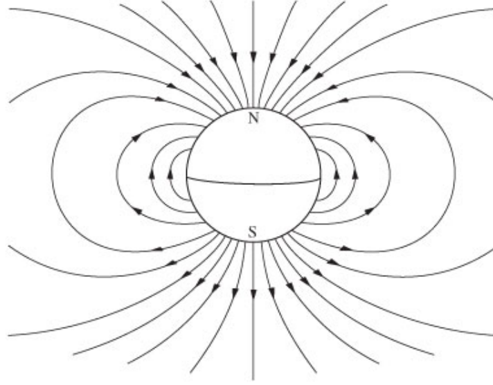
Figure 2.1.1: The magnetic dipole of the earth with a dipole moment of 8.05 \times 10^{22} \text{ A-m}^2 .
