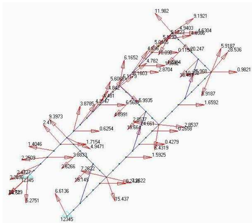
Figure 3.11: Distributed load used to scale the three-cell experiment from the N-MAS wind tunnel model.
