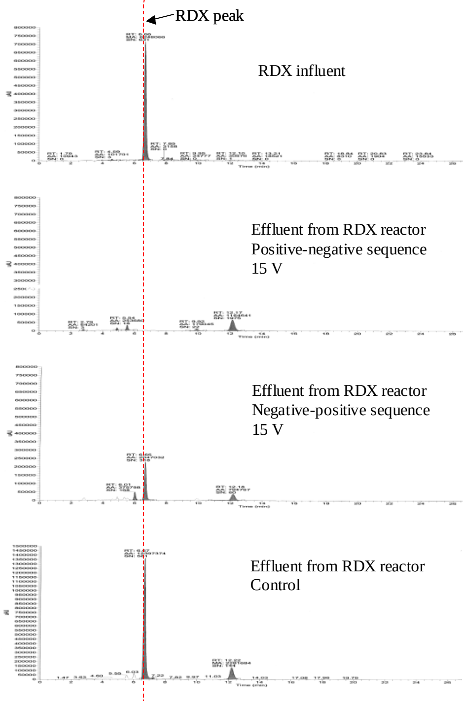
Figure 17. HPLC Chromatograms from the RDX reactors. Top: Influent Solution; 2 nd : Effluent from +- reactor; 3 rd : Effluent from -+ reactor; Bottom: Effluent from Control Reactor.
