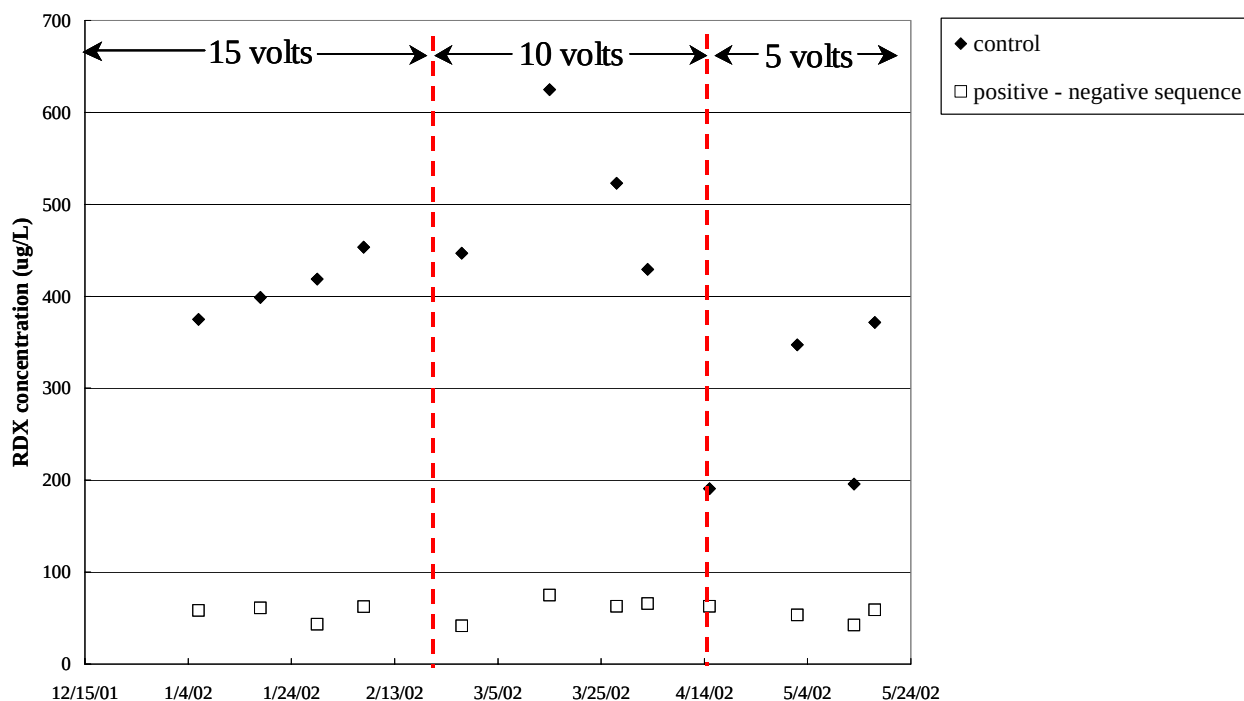
Figure 10. RDX Effluent Concentrations (GC/MS) from the Control Reactor and Positive - negative electrode sequence.
