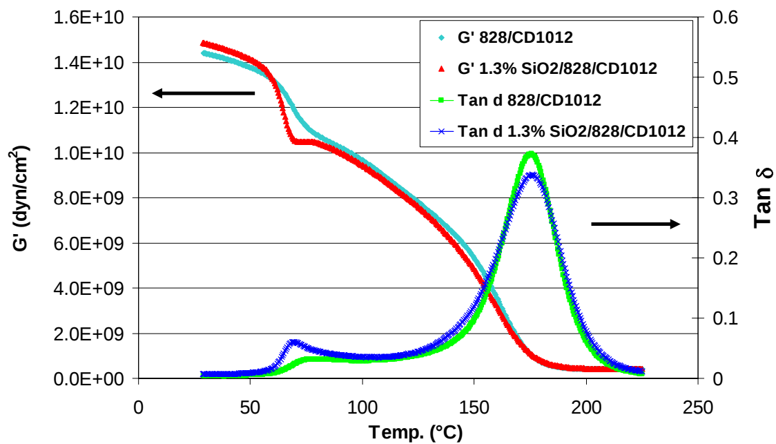
Figure 8. Dynamic storage modulus and tan \delta curves (versus temperature) of the e-beam-cured pure Epon 828/CD1012 and 1.3 wt.% \text{SiO}_2 /Epon 828/CD1012 nanocomposite.
