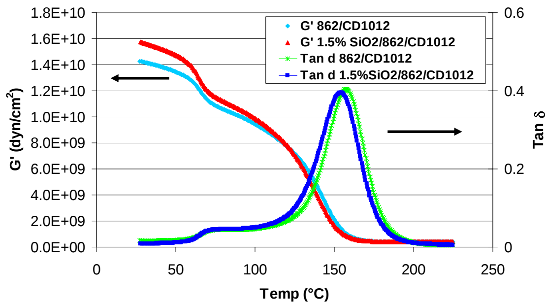
Figure 6. Dynamic storage modulus and \tan \delta curves (versus temperature) of the e-beam-cured pure Epon 862/CD1012 and 1.5 wt.% \text{SiO}_2 /Epon 862/CD1012 nanocomposite.
