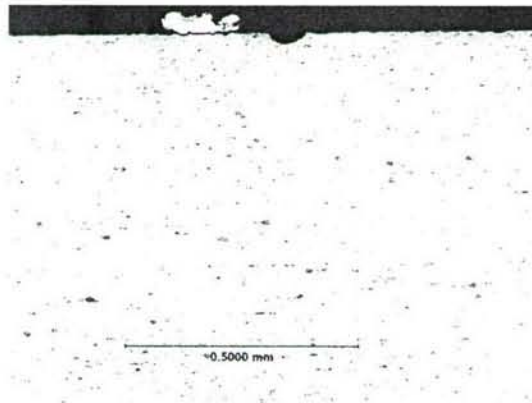
(b) 7075-T6 with Al-Zn coating
