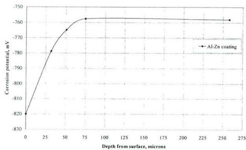
Corrosion potential profile: Plasma sprayed Al-Zn coating on 7075-T6
