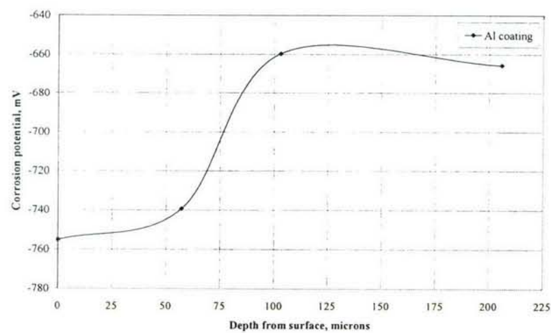
Corrosion potential profile: Plasma sprayed Al coating on 2024-T3
