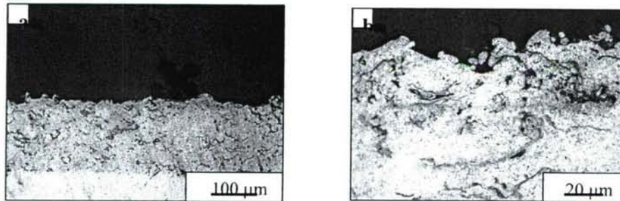
Figure 19. Plasma Sprayed Al-5Fe-5Gd Coating on 7075-T6 Substrate at (a) low and (b) high magnification
