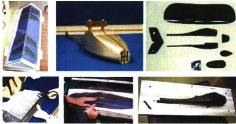
Figure 66: Manufacturing Components
