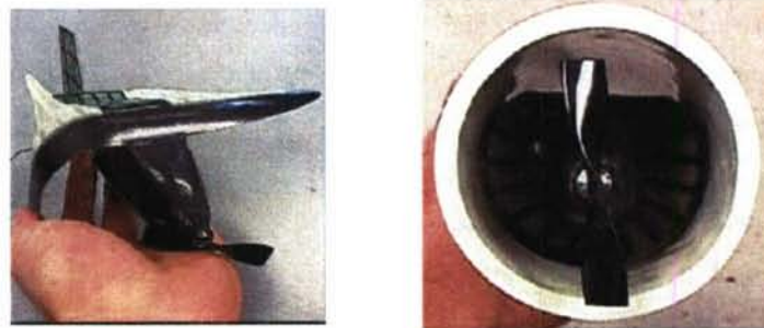
Figure 94: Rolling the MAV wing
