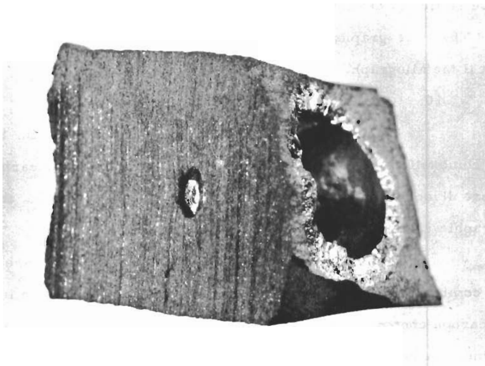
Figure 20. Section of a Melting Point Specimen Shortly Before Collapse. (Note the observation hole filled with melt)
