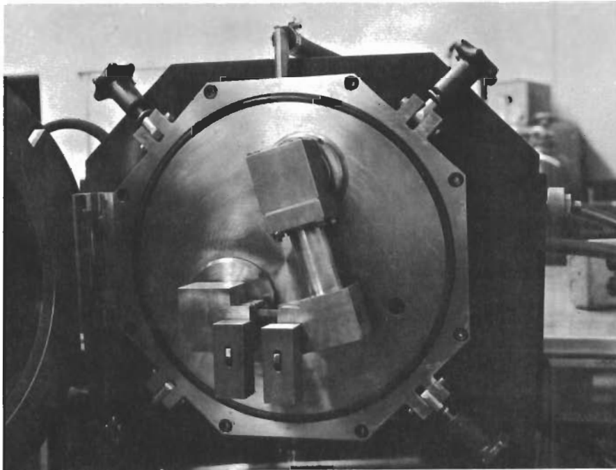
Figure 11. Interior View of the Melting Point Furnace
