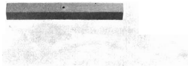
Figure 12. Pirani Melting Point Specimen, Cold-Pressed to Size and Sintered (actual size)
