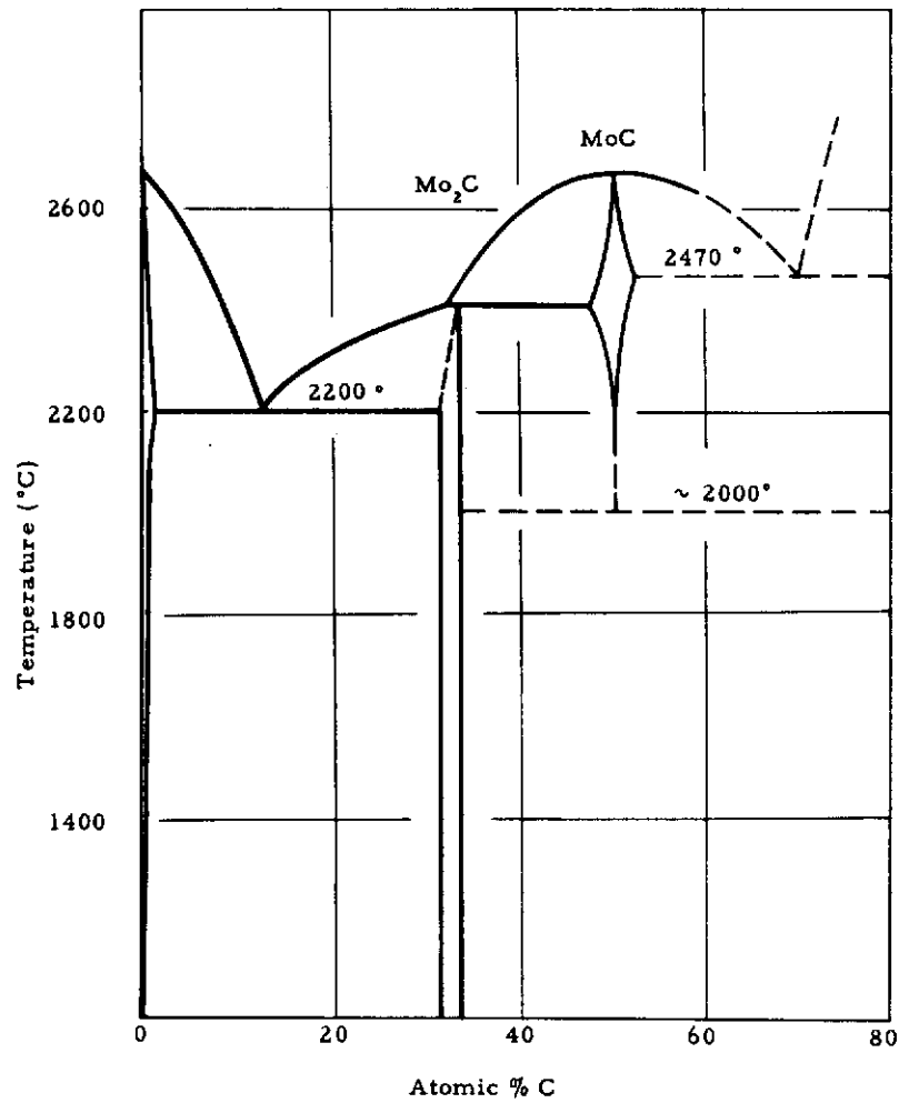
Figure 2. Molybdenum-Carbon Phase Diagram (After R. Kieffer and F. Benesovsky, 1963)
