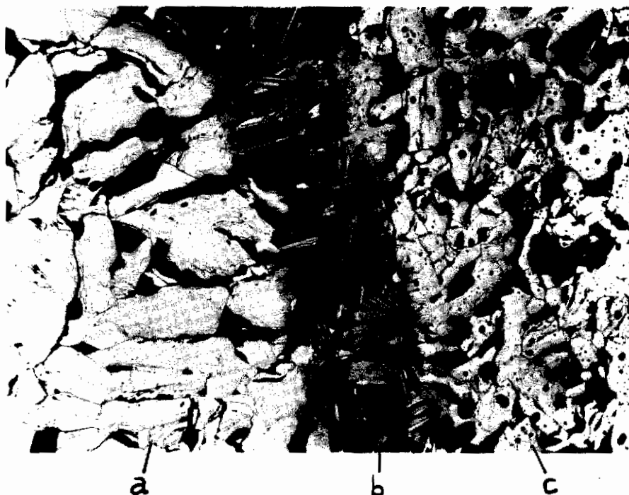
Figure 28. Mo-C (32.8 At% C), Heated Under a Temperature Gradient and Quenched X25
