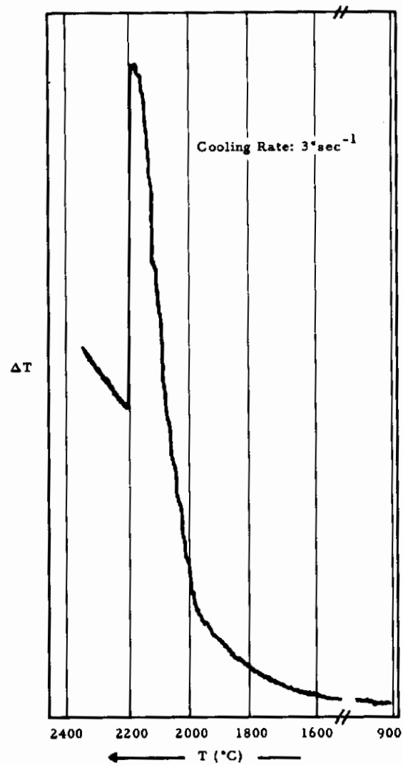
Figure 21: Differential Cooling Curve of a Molybdenum-Carbon Alloy with 20 Atomic % C
