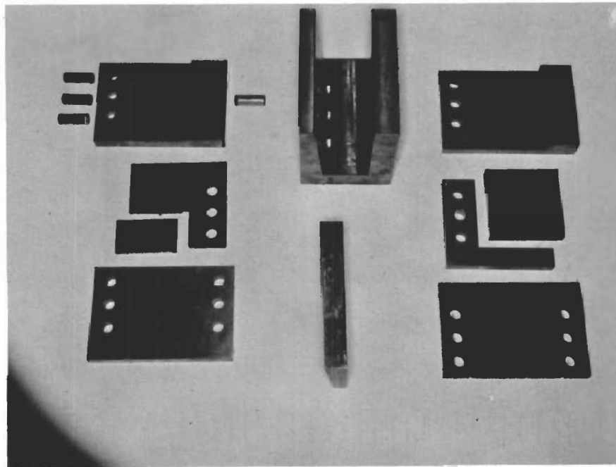
Figure 14. Die Components for Cold-Pressing Pirani Melting Point Specimens
