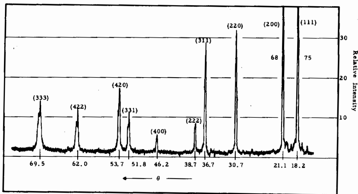
Figure 52. Diffraction Pattern of the Cubic (B1) High Temperature Phase in the System Molybdenum-Carbon
