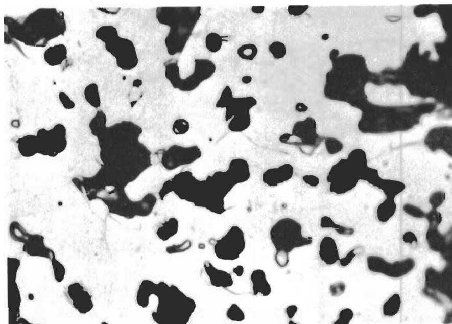
Figure 37. Mo-C (38At% C), Quenched from 2500°C. X1000 Single Phase \eta -MoC 1-x with Pores (Black)
