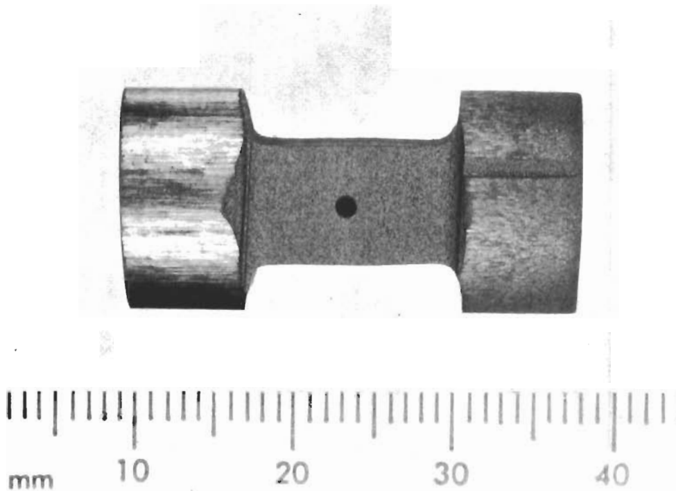
Figure 13. Pirani Melting Point Specimen, Hot Pressed and Ground
