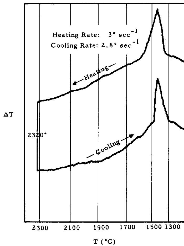
Figure 32. Differential Heating and Cooling Curve of a Molybdenum-Carbon Alloy with 33 Atomic % Carbon
