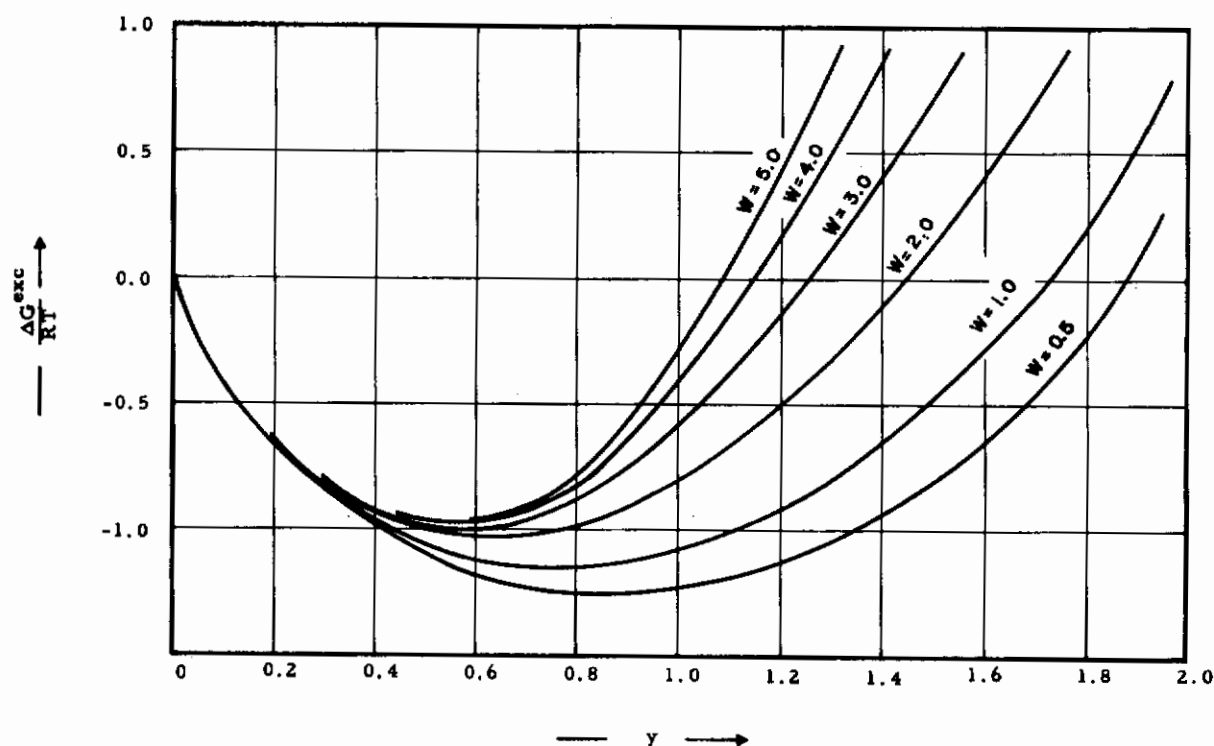
Figure 63. Model 2. Excess Free Energy due to Disorder in the Carbon Sublattice. Parameter: w = \frac{\Delta E}{RT} (Quantities per Mole \text{Me}_2\text{C}_y )
