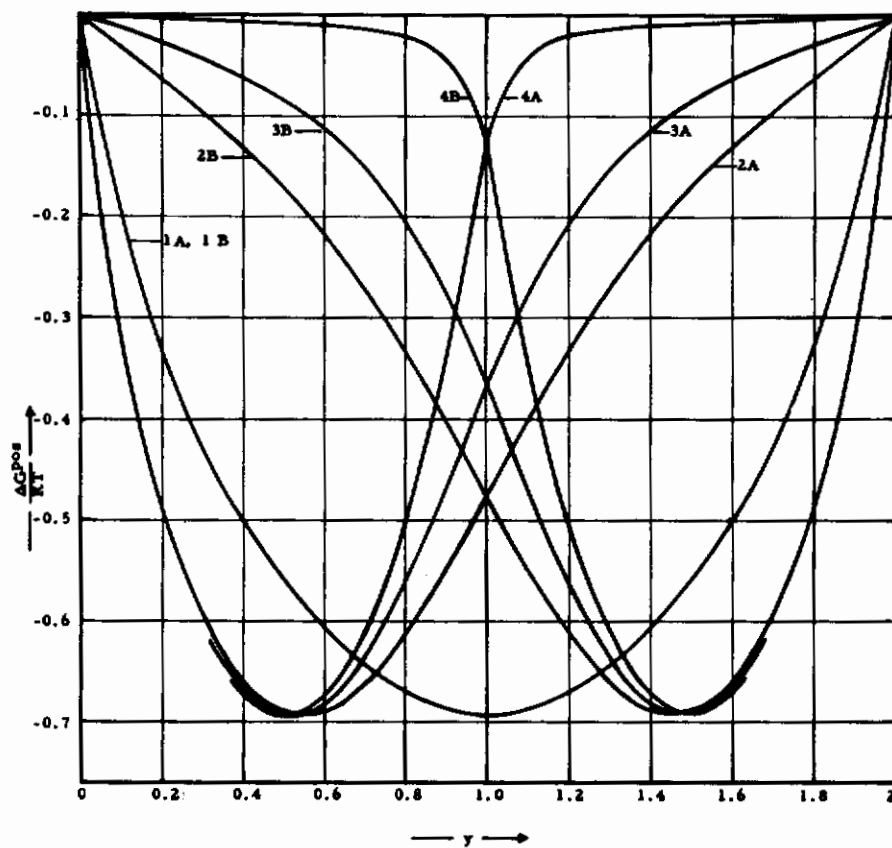
Figure 66: Model 1: Individual Contributions of the Interstitial Sublattices to the Positional Free Energy of a Two-Level System.
