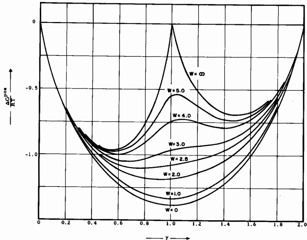
Figure 69. Model 2: Positional Free Energy Resulting From the Distribution of Interstitial Atoms Among Two Types of Interstitial Lattice Sites.
