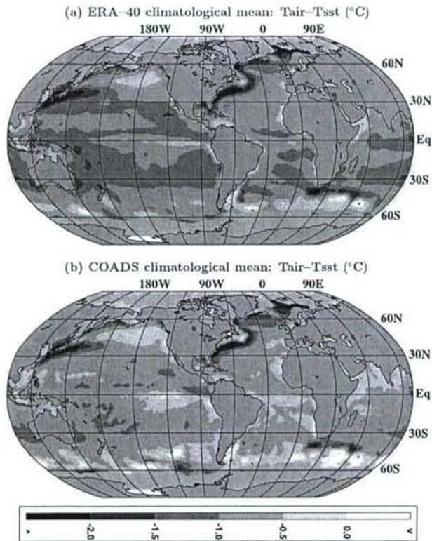
Figure 1. Climatological mean air–sea surface temperature differences over the global ocean as obtained from (a) ERA-40 and (b) COADS. Construction of both data sets are described in section 2. Tair–Tsst values at high latitudes (Arctic and Antarctic) will not be used in this paper due to the existence of ice.
