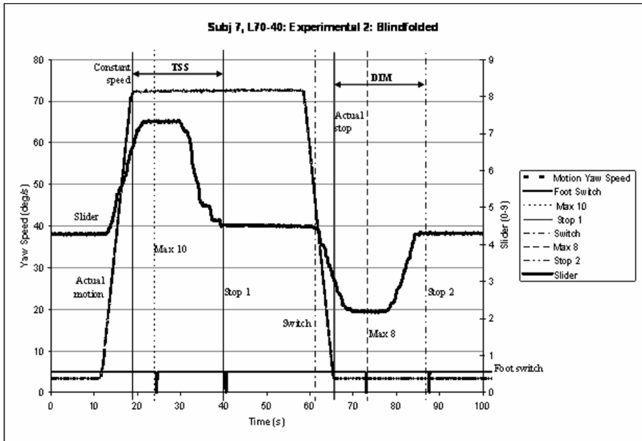
Figure 1. A graph of a counterclockwise (left) spin at 70 degrees/second for 40 seconds. Initial and subsequent max velocities, actual and perceived stopping points, and the switch in direction are marked by vertical lines as indicated in the legend. The TSS is measured from the beginning of the actual profile's plateau to the first perceived stop. DIM, the time from the cessation of actual motion until the perception of rotation in the opposite direction ends is measured from the end of the profile to the second perceived stop.
