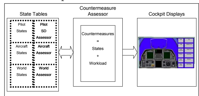
Figure 3. Spatial disorientation aiding system architecture.
