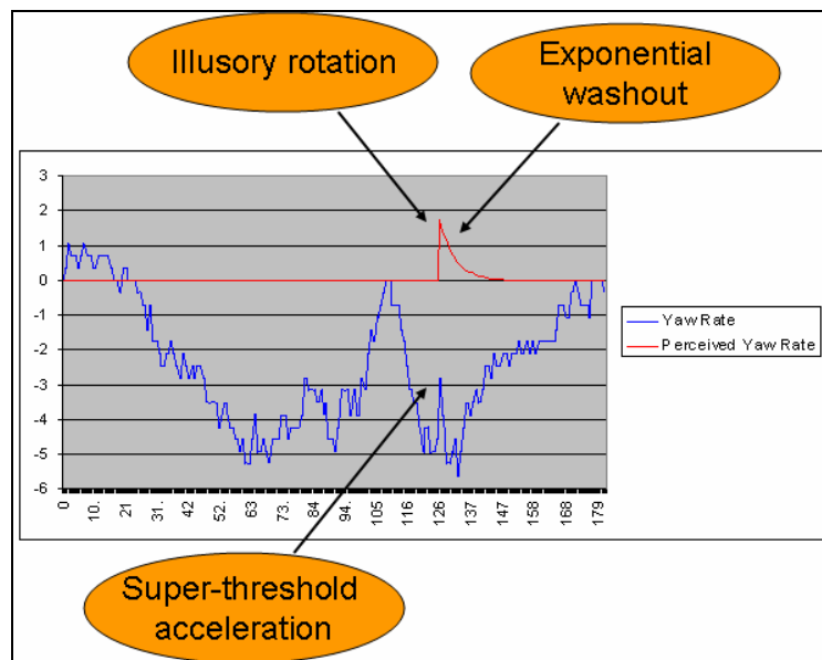
Figure 8. Actual vs. perceived yaw rate example 1.
