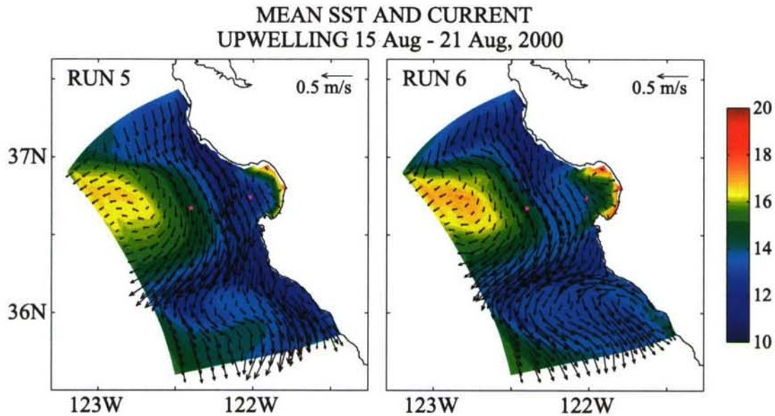
Figure 9. The NCOM ICON model predicted SSTs (averaged over the upwelling event) from runs 5 and 6 (Table 1) forced with corresponding COAMPS wind stresses from the Figure 8.
