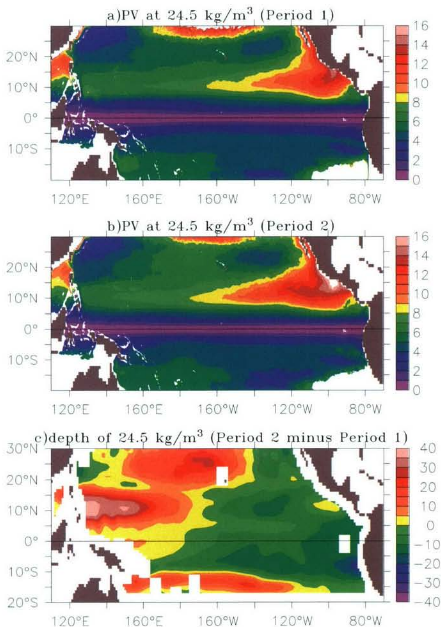
FIG. 4. Absolute value of potential vorticity ( 10^{-10} \text{ m}^{-1} \text{ s}^{-1} ) on the 24.5\text{-}\sigma_{\theta} surface averaged for (a) Period 1 and (b) Period 2. (c) Difference in the mean depth of the 24.5\text{-}\sigma_{\theta} surface for Period 2 minus Period 1.
