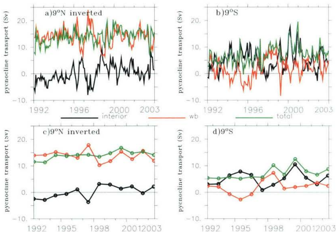
FIG. 3. Pycnocline volume transport at 9^{\circ}\text{N} and 9^{\circ}\text{S} as a function of time. The results at 9^{\circ}\text{N} are inverted for easy comparison. (a), (b) Monthly data and (c), (d) annual averages of the monthly means are shown. Black, red, and green lines represent the interior ocean, western boundary, and total across the basin transport, respectively. The interior ocean and western boundary subdomain is separated by 145^{\circ}\text{E} ( 160^{\circ}\text{E} ) for the transport at 9^{\circ}\text{N} ( 9^{\circ}\text{S} ).
