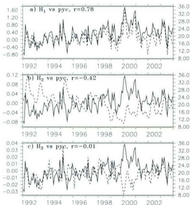
FIG. 12. Relationship between pycnocline volume transport convergence across 9^{\circ}\text{N} and 9^{\circ}\text{S} (solid lines, units: Sv, using the right y axis) and heat transport divergence across the same latitudes (dashed lines, units: PW, using the left y axis, negative means convergence). Heat transport divergence is decomposed into contributions from anomalous circulation and thermal anomalies (named as H_1 , H_2 , and H_3 ) according to Eqs. (2)–(4) in the text. The correlation coefficient between the two time series in each panel is marked.
