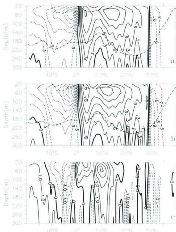
FIG. 1. Meridional overturning circulation in the top 300 m of the model (Sv). Solid (dashed) lines indicate clockwise (counter-clockwise) circulations. Dashed-dotted lines indicate the 22.5 and 25.3 \sigma_\theta surfaces. Mean state for (a) Period 1 (defined in the text), (b) Period 2 (defined in the text), and (c) the difference between Periods 1 and 2, (b) minus (a), are shown.
