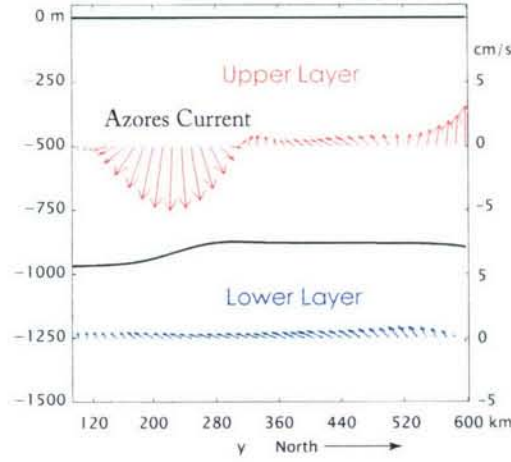
Figure 3-9: A cross-section of the velocity profile in the open ocean interior x=200\text{km} (dashed line in Figure 3-8). In the upper layer, an eastward zonal jet forms at about y=220 \text{ km} with a maximum velocity of 5 \text{ cm s}^{-1} and a westward flow forms along the northern boundary with a maximum velocity of 3 \text{ cm s}^{-1} . The lower layer shows a weak westward flow near the northern boundary. The interface, superimposed on the figure, tilts up to the northward (+ y direction) below the eastward jet.
