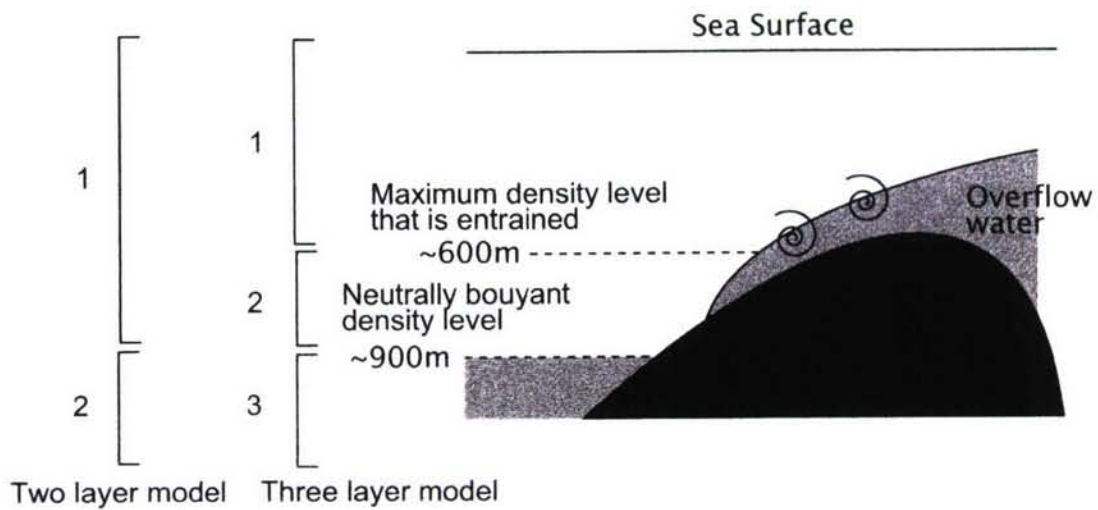
Figure 3-23: A schematic of how the layer interfaces are configured in the two and three layer model. The two-layer model splits the overflow and the upper layer by setting the density of the overflow water to that of the product water. The interface between the overflow water and the upper ocean water is about 900 m in the open ocean. The three-layer model further splits the upper layer of the two-layer model into two at the maximum density level that is entrained to the overflow. This isopycnal is about 600 m in the open ocean. The new middle layer is not forced diabatically but interacts with other layers through pressure.
