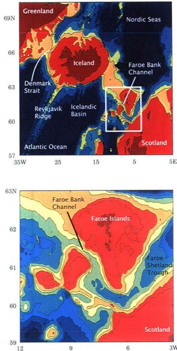
Figure 1-7: Map of Northern Atlantic (above) based on Smith and Sandwell's bottom bathymetry (Smith and Sandwell, 1997). The bathymetric contours are shown from 0 to 2000 m every 500 m. The Denmark Strait (west) and the Faroe Bank Channel (east) are the two deep straits known to connect the Nordic Seas and the North Atlantic. The Denmark Strait is located between Greenland and Iceland. The Faroe Bank Channel is located between Iceland and Scotland. Figure below shows a closer look of the region near the Faroe Bank Channel. The bathymetric contours are from 0 to 1000 m every 200 m. The upstream basin of the Faroe Bank Channel overflow is the Faroe-Shetland Trough and the overflow flows into the Atlantic through the Faroe Bank Channel which is about 800 m deep.
