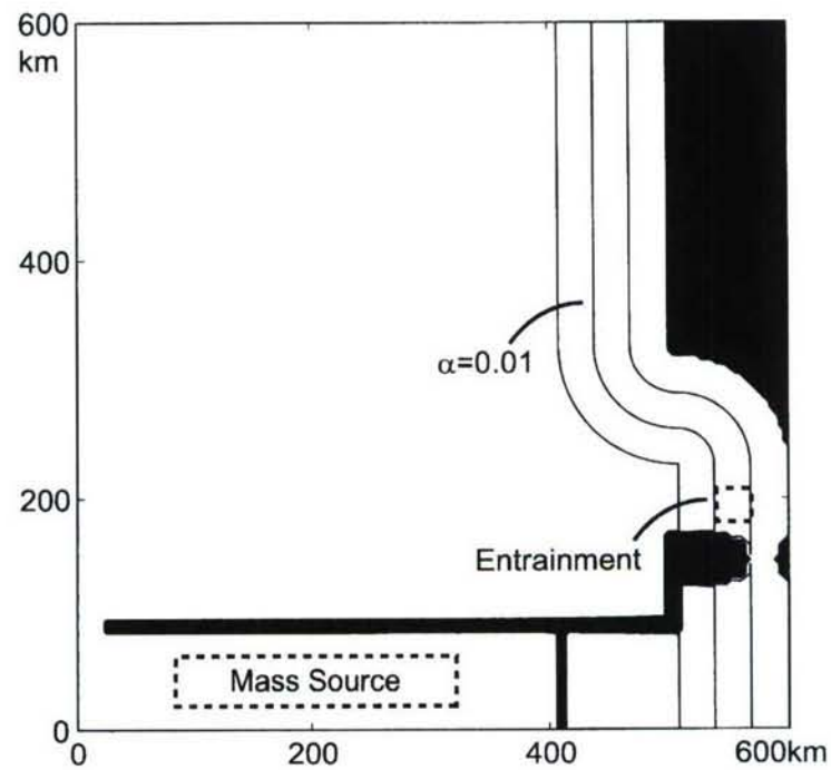
Figure 3-5: The bottom bathymetry for Case 6 where a curvature is added to the slope of Case 5 (Figure 3-3). The slope is kept to 0.01, a constant and the spatial scale of the curvature is 100 km and is close to that of the curvature between the Gibraltar Strait and the steep slope region near Cape St. Vincent. Other parts of the model are the same as Case 5.
