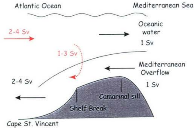
Figure 1-9: A schematic of the mass balance of the Mediterranean overflow(right) and the Atlantic Ocean(left). Camarinal sill separates the two regions. Overflows spills into the open ocean from the marginal sea with a transport of 1 Sv at the Camarinal sill. An equivalent amount of mass returns to the marginal sea in the upper layer. The overflow transport increases to 2–4 Sv by Cape St. Vincent. This increase of overflow water indicates entrainment of 1–3 Sv which is know to occur near the shelf break. The mass balance, therefore, indicates that the upper layer must flux 2–4 Sv into Gulf of Cadiz. Black arrows indicate directly observed estimates whereas red arrows indicate indirect estimates.
