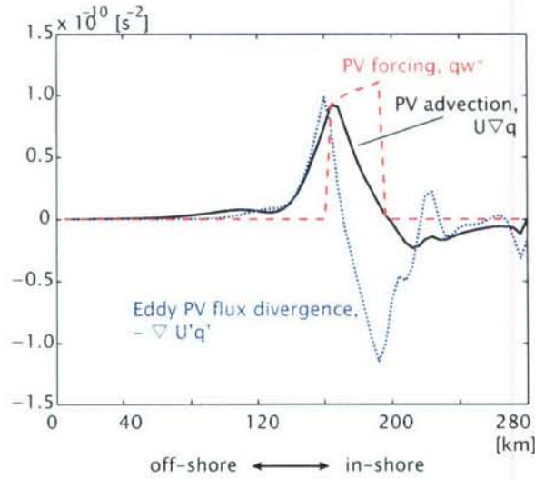
Figure 2-22: PV Balance near the entrainment region, \bar{U} \cdot \nabla \bar{q} = \bar{q}w^* - \nabla \cdot \bar{U}'q' . The eddy PV flux divergence (blue dotted line, \nabla \cdot \bar{U}'q' ) is positive off-shore and negative on-shore. This is due to baroclinic instability (Case 3). The entrainment is a PV forcing (red dashed, \bar{q}w^* ) and the mean PV advection (black solid line, \bar{U} \cdot \nabla \bar{q} ) is forced by the sum of the PV increase by entrainment and the eddy PV flux divergence created by the baroclinic instability. Regions of both negative mean PV advection and positive mean PV advection exist which leads to the double gyre topographic \beta -plume.
