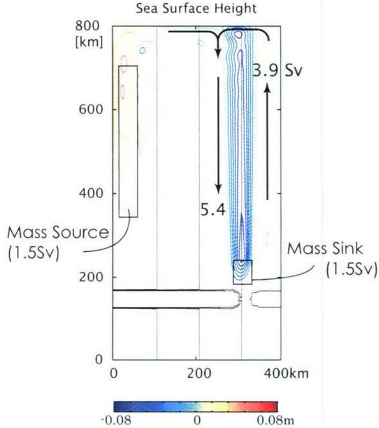
Figure 2-3: The sea surface height responding to the mass sink (entrainment) located in the square boxed region near the strait. The diapycnal velocity of the mass sink is w^* = 7.8 \times 10^{-4} \text{ m s}^{-1} . The flow field shows the cyclonic circulation along the constant bathymetric contours (background PV contours) which is the entrainment-driven topographic \beta -plume. A flow up the PV gradient is forced at the mass sink and a flow down the PV gradient is created at the northern boundary. The inflow to the mass sink has a transport of 5.4 Sv and the outflow has a transport of 3.9 Sv, close to the estimate from Eq 2.12. A mass source (Return mass flux) is located in the off shore location with w^* = 1.2 \times 10^{-4} \text{ m s}^{-1} to conserve mass in the upper layer and this mass source creates the anticyclonic gyre off-shore.
