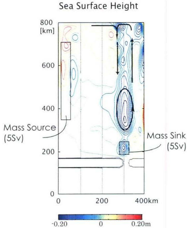
Figure 2-4: The sea surface height of the topographic \beta -plume when w^* = 2.5 \times 10^{-3} \text{ m s}^{-1} \gg w_c . The model setup is exactly the same as the case shown in Figure 2-3 except for this diapycnal velocity strength. Contours are drawn from -0.2 to 0.2 m with an interval of 2.5 cm. The eddies form near the forcing region and the main structure of the topographic \beta -plume is broken into cyclonic eddies. The eddies have a velocity as large as 40 \text{ cm s}^{-1} .
