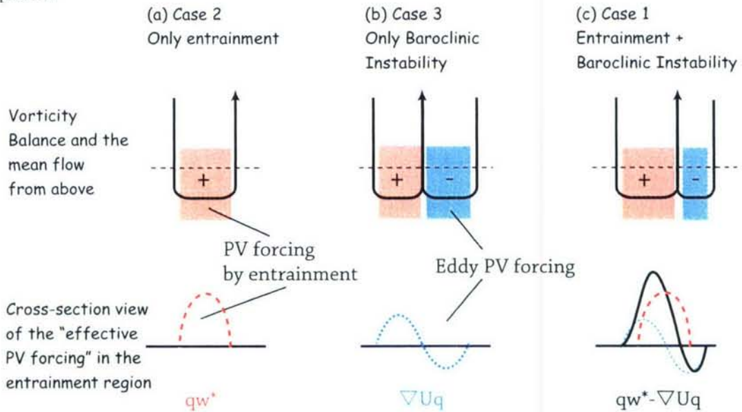
Figure 2-22: PV Balance near the entrainment region, \bar{U} \cdot \nabla \bar{q} = \bar{q}w^* - \nabla \cdot \bar{U}'q' . The eddy PV flux divergence (blue dotted line, \nabla \cdot \bar{U}'q' ) is positive off-shore and negative on-shore. This is due to baroclinic instability (Case 3). The entrainment is a PV forcing (red dashed, \bar{q}w^* ) and the mean PV advection (black solid line, \bar{U} \cdot \nabla \bar{q} ) is forced by the sum of the PV increase by entrainment and the eddy PV flux divergence created by the baroclinic instability. Regions of both negative mean PV advection and positive mean PV advection exist which leads to the double gyre topographic \beta -plume.
