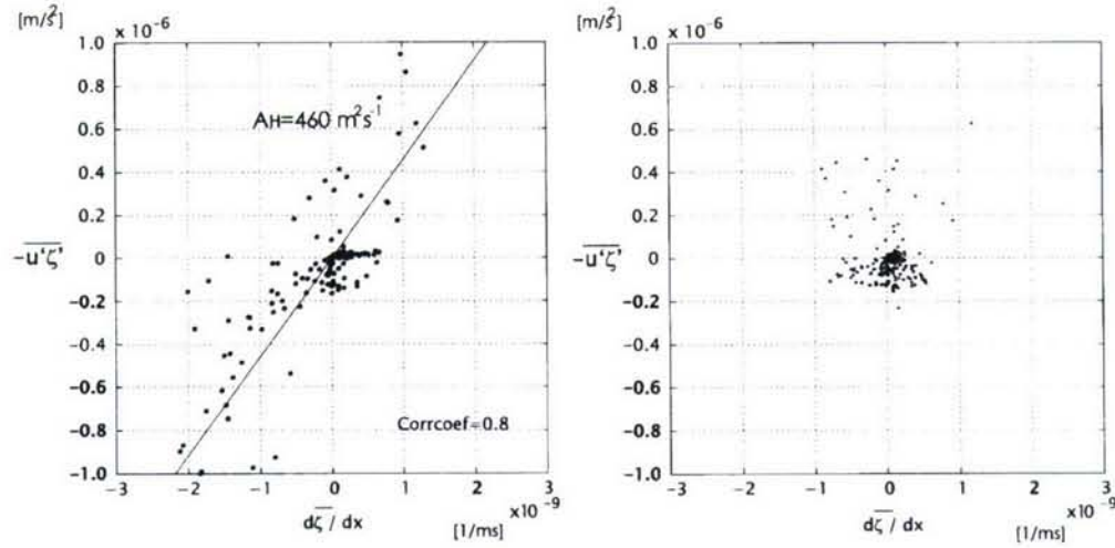
Figure 3-22: The Reynolds Stress in the across-slope direction ( -\overline{u'\zeta'} ) plotted against the mean vorticity gradient across-slope ( \bar{\zeta}_x ) in the steep slope region. The ratio of the two terms ( \frac{-\overline{u'\zeta'}}{\bar{\zeta}_x} ) is the estimate for the viscosity coefficient ( A_H^* ) for each point thus the slope of the best fit line will give the rough estimate for the viscosity coefficient in the region. (a) The region where slope varies from 0.01 to 0.04 (Figure 3-21a) Though the orientation of the slope changes with location, -\overline{u'\zeta'} and \bar{\zeta}_x are estimated so that the eddy momentum flux are the values in the cross-slope direction and the vorticity gradient in the cross-slope region respectively. There is reasonable correlation between the two terms, with a correlation coefficient of 0.8, and the viscosity coefficient estimates to be about 460 \text{ m}^2 \text{ s}^{-1} . (b) The region where slope is constant ( \alpha = 0.01 ). The Reynolds Stress is still of significant size but there is no significant correlation with the mean vorticity gradient. The eddies do not appear to be strongly fluxing momentum down-gradient of the mean in this region.
