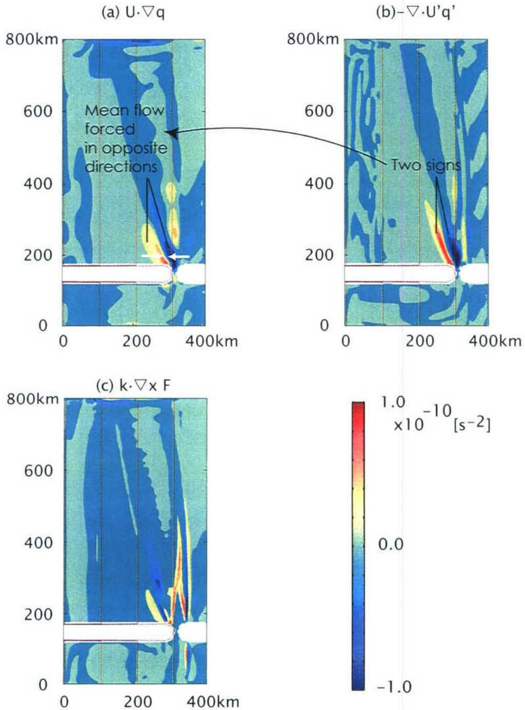
Figure 2-15: Each of the terms in Vorticity equation: Eq 2.27. (a) PV advection term ( U \cdot \nabla q ) (b) Eddy PV flux divergence term ( -\nabla(U'q') ) and (c) Dissipation term ( \hat{k} \cdot \nabla \times F ). The above balance shows (a) and (b) having two signs and balancing each other near the strait. This is the main balance of the eddy-driven topographic \beta -plume. The two signs show that the mean flow is bi-directional, making the time-mean circulation double gyre structure. The dissipation term shows large values where the interface intersects the bottom topography.
