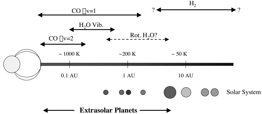
Fig. 1. A schematic of a protoplanetary accretion disk around a classical T Tauri star is shown with respect to the radial location of planets in the Solar System and known extra-solar planets. Approximate dust continuum temperatures are indicated at fiducial radii. At a radius of several stellar radii, the disk is truncated by a stellar magnetosphere, and material accretes onto the star along the field lines. The approximate radial locations of emission line diagnostics discussed in the text are shown.
