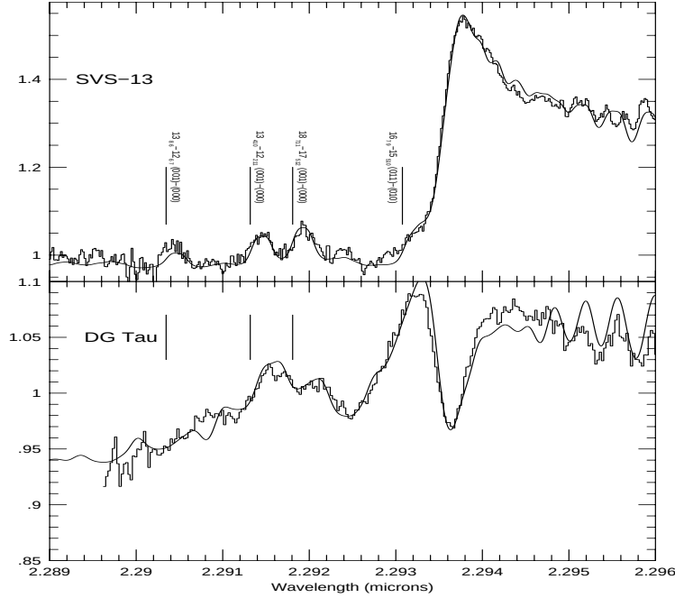
Fig. 4. Hot \text{H}_2\text{O} emission in the young stellar object SVS-13 and the classical T Tauri star DG Tau. The histograms are the observed spectra, and the smooth lines are disk models of the spectra. In SVS-13, the molecular emission is relatively narrow, and individual ro-vibrational transitions of \text{H}_2\text{O} can be resolved; identified transitions are labeled. Emission from the CO v=2-0 bandhead is seen at wavelengths longer than \sim 2.2934\mu\text{m} . In DG Tau, the \text{H}_2\text{O} emission lines are blended due to the rotational broadening; the double-peaked profile is most evident at \approx 2.2918\mu\text{m} . The dip in the CO bandhead at \sim 2.2936\mu\text{m} is caused by CO absorption in the late-type stellar photosphere of DG Tau.
