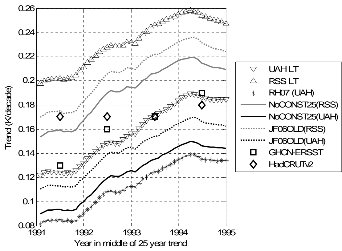
Figure 6.1 25-year LTP for various estimated troposphere temperature trends.
