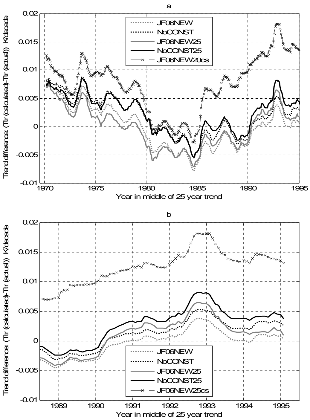
Figure 4.11 Same as figure 4.9 with 25-year time periods
