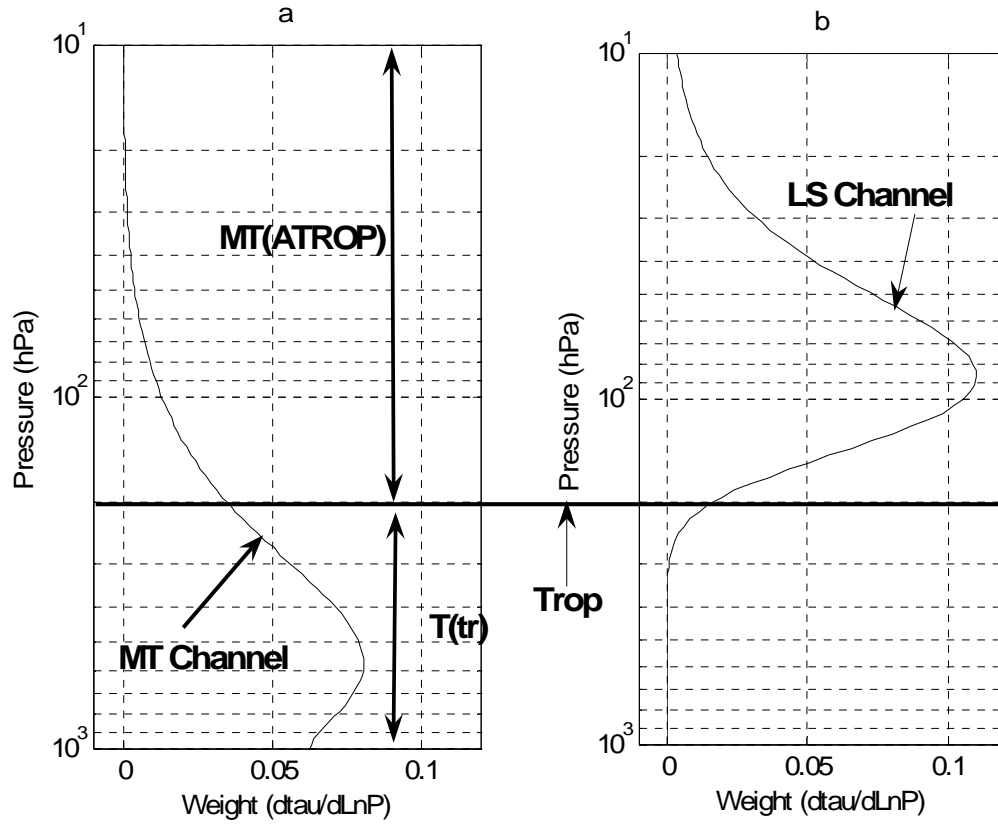
Figure 4.5 (a) MT weighting function. RH07 subtracts the layer above the tropopause (MT(ATROP)) from the entire MT channel to estimate the tropospheric layer ( T_{TR} ). (b)
