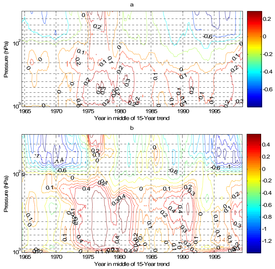
Figure 4.2 (a) 15-year Limited time period trends (K/decade) on globally averaged RATPAC(RW) data, (b) Tropical (20°N-20°S)
