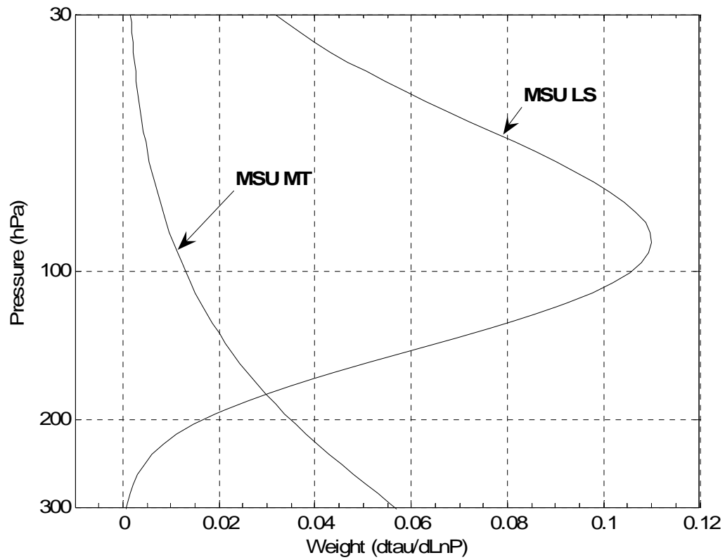
Figure 4.1. Layer where the MSU LS and MT weighting function intersect. MT has contribution from the stratosphere (above 200 hPa for global average).. The biggest impact for a combination of the two channels is between 100 hPa and 200 hPa, the region of greatest variability in the ZTL.
