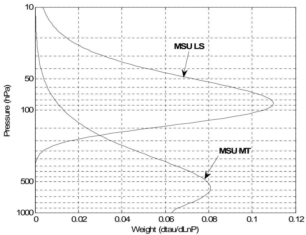
Figure 2.1 MSU LS and MT Weighting functions
