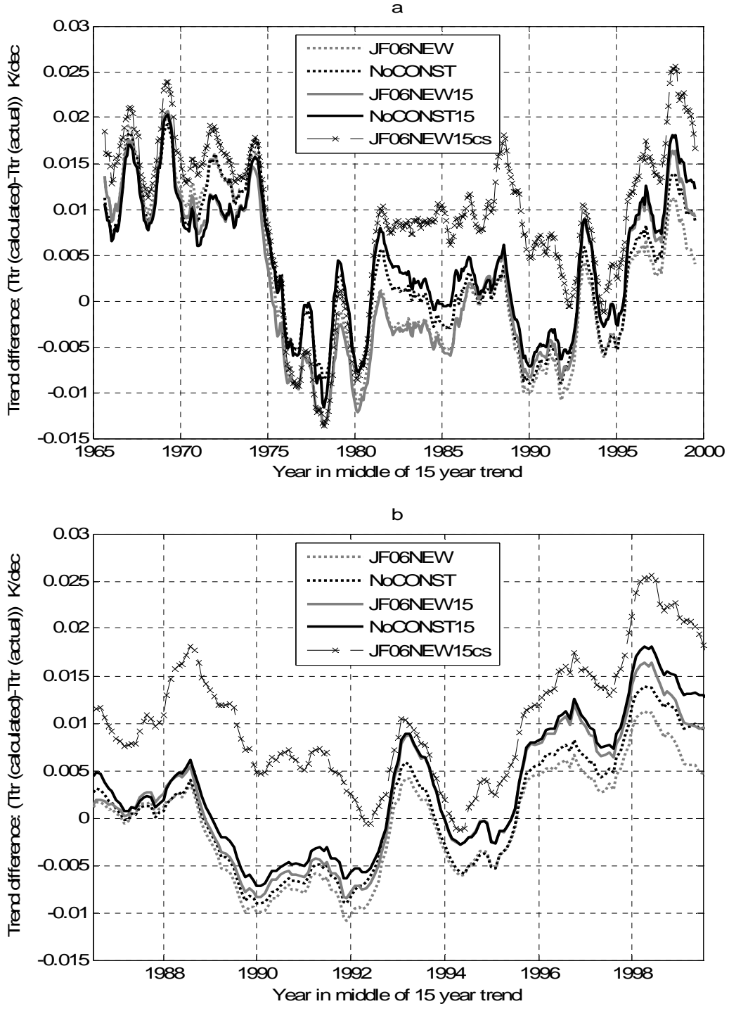
Figure 4.9 (a) Various methods of creating coefficients from RATPAC(RW) radiosonde data and corresponding T_{TR} were created using equation (4.1). These were subtracted from the actual T_{TR} found using equation (4.2) for 15-year LTP over the entire radiosonde time period. (b) Over the MSU era
