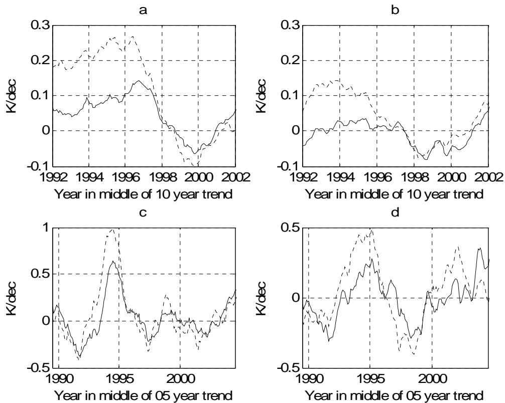
Figure 5.5 (a) 10-year LTP trends on UAH(LT)-UAH(MT) (solid) and RSS(LT)-RSS(MT) (dashed) for global, (b) tropics. (c) and (d) same as (a) and (b) for 5-year LTP trends.
