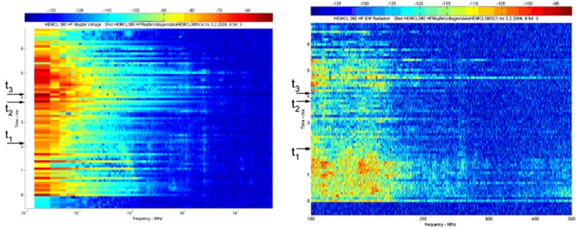
Figure 5. Spectrogram of HEMCL 380 : high-frequency muzzle voltage (left) and EM radiation (right).
