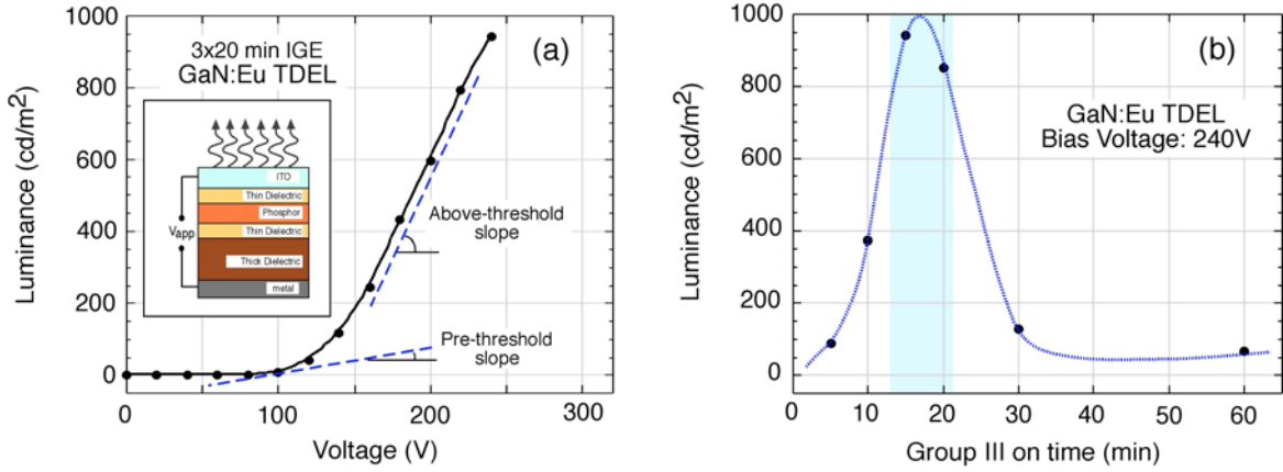
Fig. 6 (a) Luminance-voltage measurements for 3×20 min IGE GaN:Eu TDEL device. Insert shows a cross sectional view of the TDEL device. (b) luminance variation with different IGE group III ON times in GaN:Eu TDEL devices.
