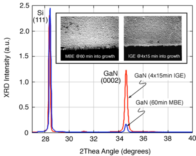
Fig. 3 XRD spectra for un-doped GaN epi layers using conventional MBE growth and 4×15 min IGE growth. SEM microphotographs of un-doped GaN epi layers using conventional MBE growth and 4×15 min IGE growth are shown in the
