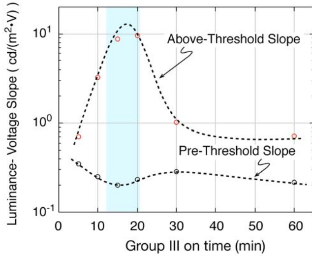
Fig. 7 Device luminance-voltage slope measured at pre-threshold and above-threshold luminance for IGE GaN:Eu TDEL devices using films grown with different group III ON times. The TDEL devices were driven using bipolar square waveform at 1kHz.
