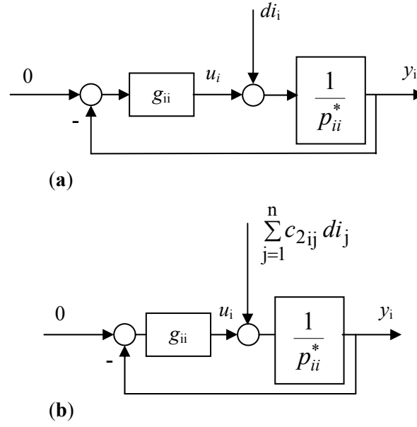
Fig. 7 i-th equivalent MISO systems
