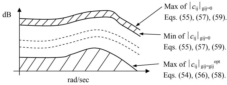
Fig. 10 Coupling effect bands with different non-diagonal controllers
