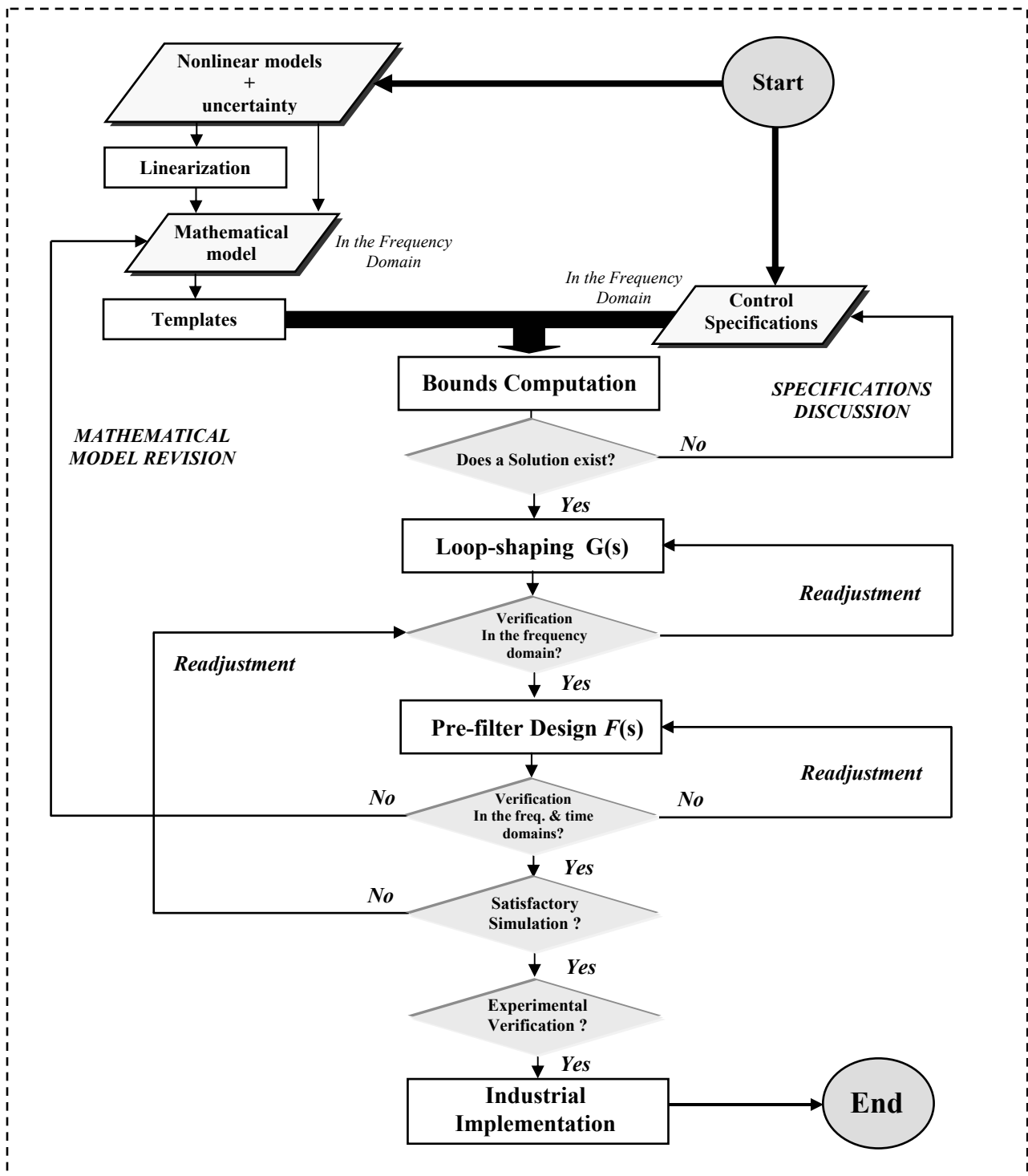
Figure 4: QFT methodology
