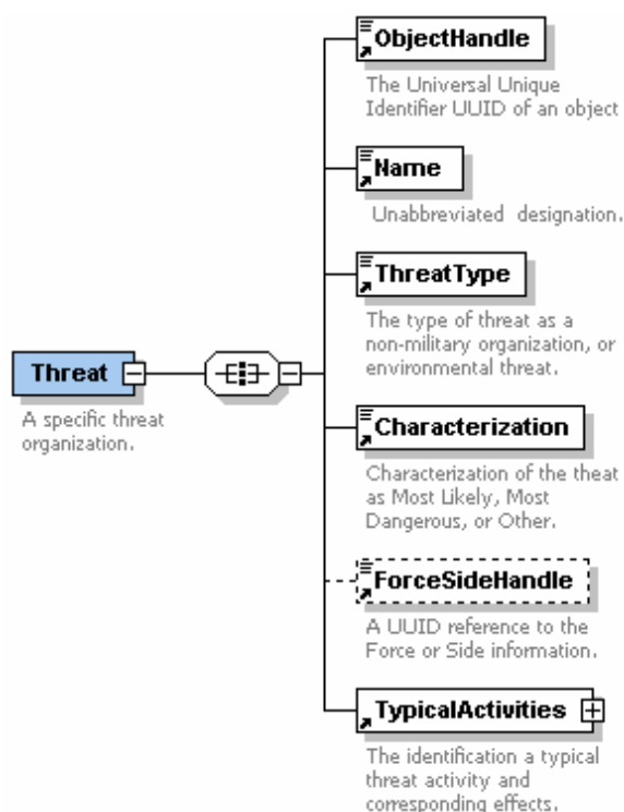
Figure 6. MSDL Threat Data Model (SISO 2005).
