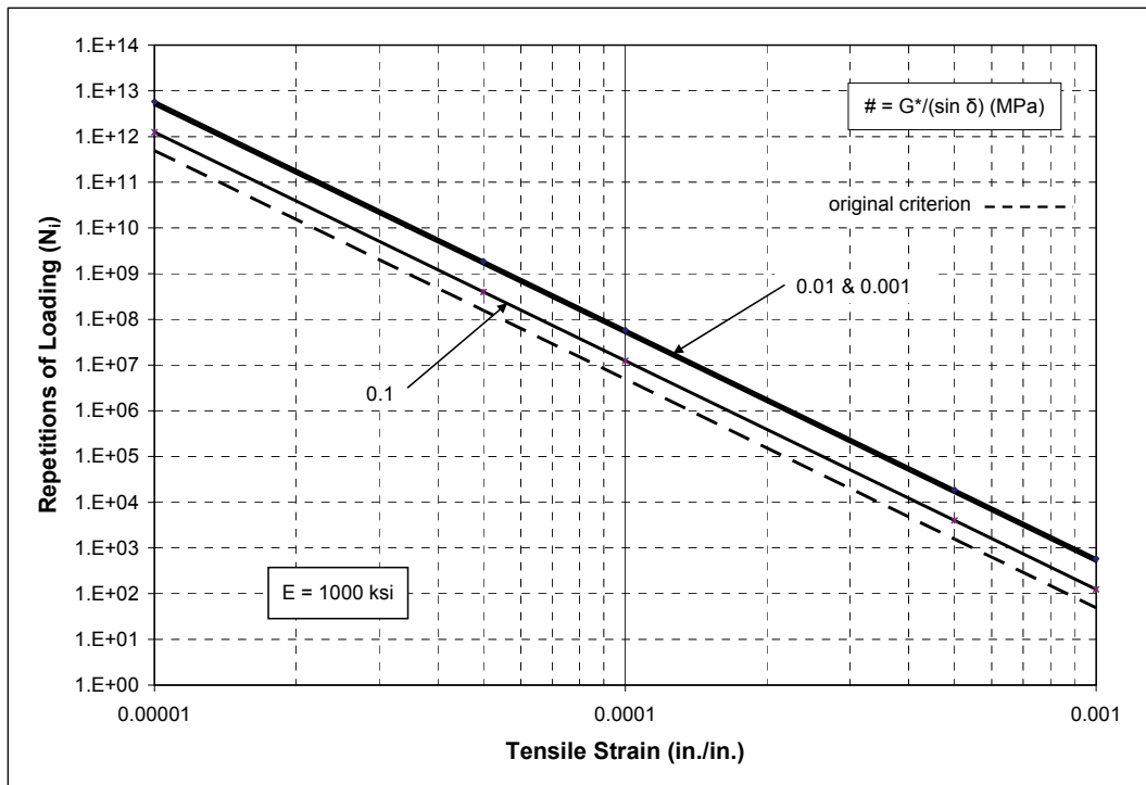
Figure 39. Preliminary adjusted criterion for aged asphalt with elastic modulus = 1000 ksi; criterion adjustment is based on both elastic modulus and G^*/(\sin \delta) .
