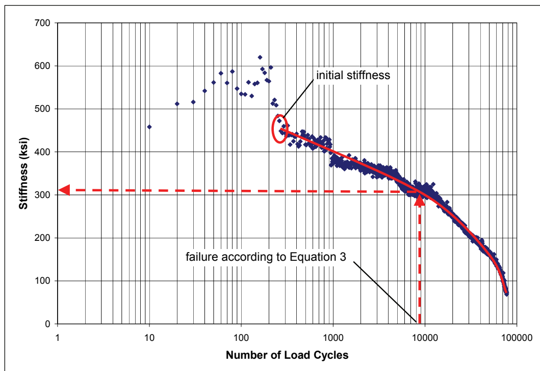
Figure 22. Establishing percent stiffness at failure for the laboratory-produced standard airfield mixture (LM), replicate 1.
