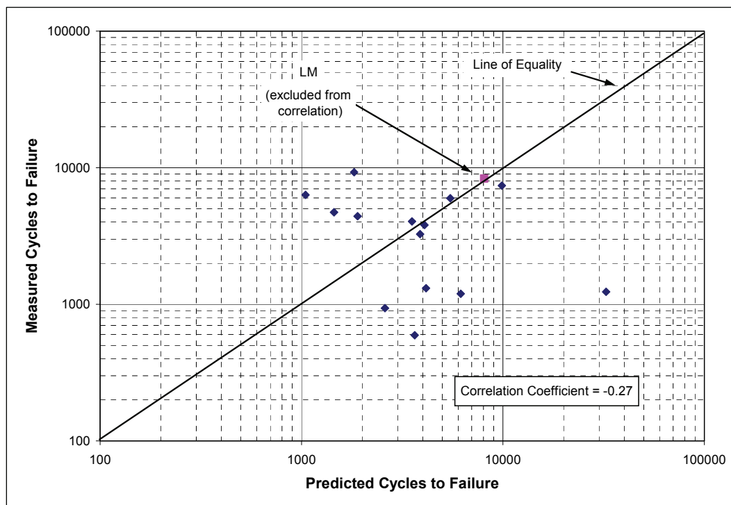
Figure 25. Comparison of predicted and measured cycles to beam fatigue failure.
