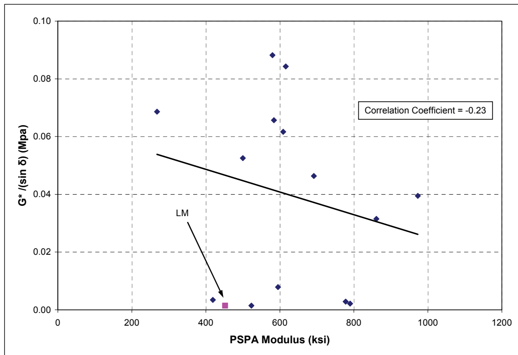
Figure 27. Relationship between PSPA modulus and G^* / (\sin \delta) .
