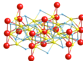
Figure 4 Fluoroapatite
