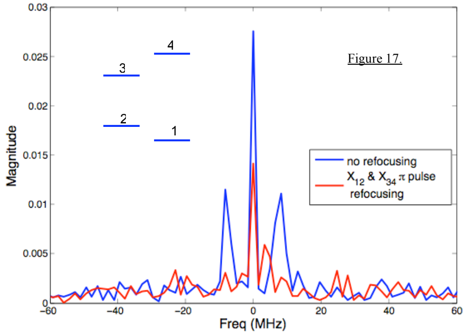
Projected magnitude of FFT wrt \tau
