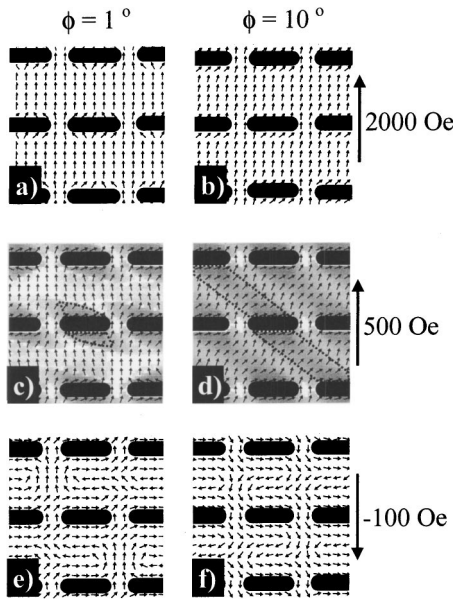
FIG. 7. Micromagnetic domains vs H (2000, 500, and -100 Oe) and angle \phi ( 1^\circ and 10^\circ ). In panels (c) and (d) a gray-scale proportional to the magnetization component perpendicular to the short axis of the ellipses is used to highlight the domain structure. The dotted lines are a guide to the eye.
