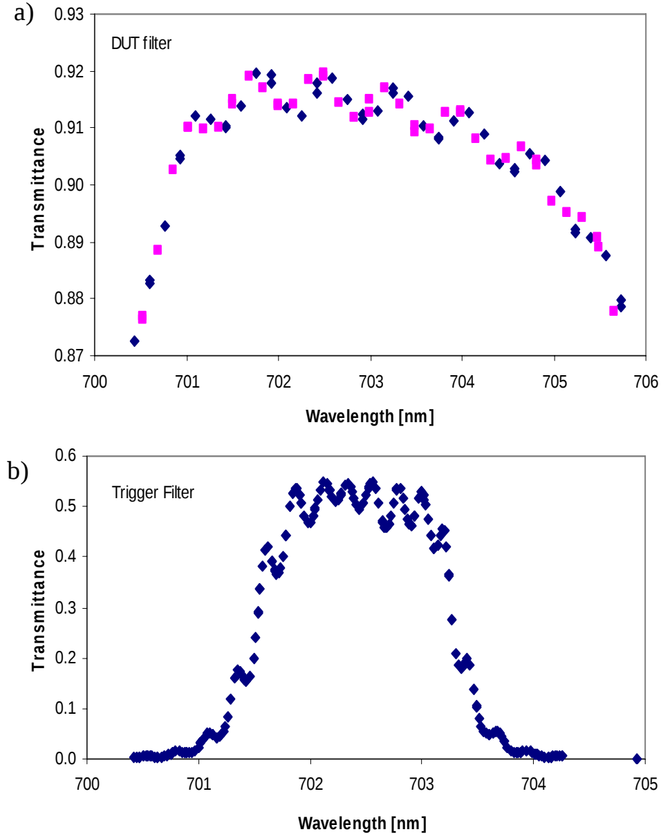
Fig. 9. Transmittance spectra of filters measured with SIRCUS. a) FDUT: two measurements (squares, diamonds) taken \sim 1 hour apart. b) FT.
