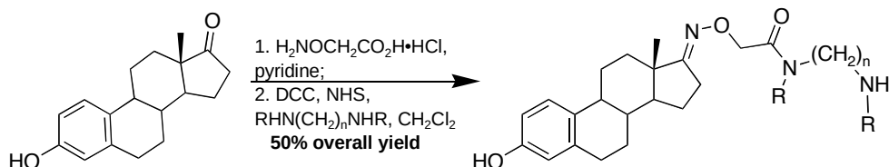
Scheme 1. In this case, compounds have been made with R=H or CH 3 and with n=2 or 6.
