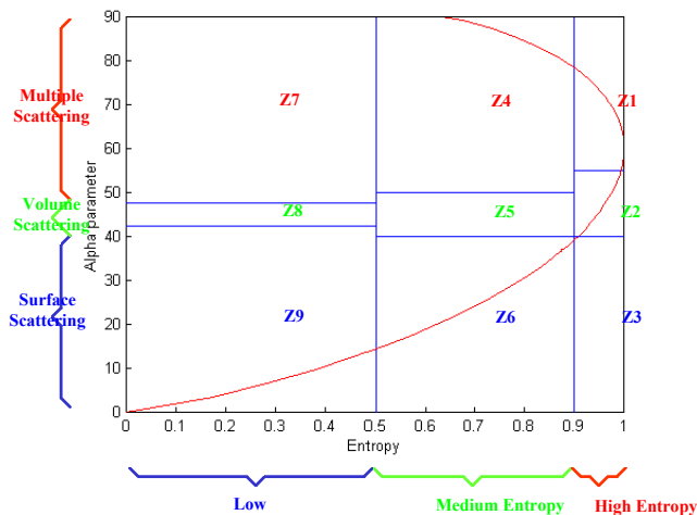
Fig. 13a : The H / \underline{\alpha} classification plane.
