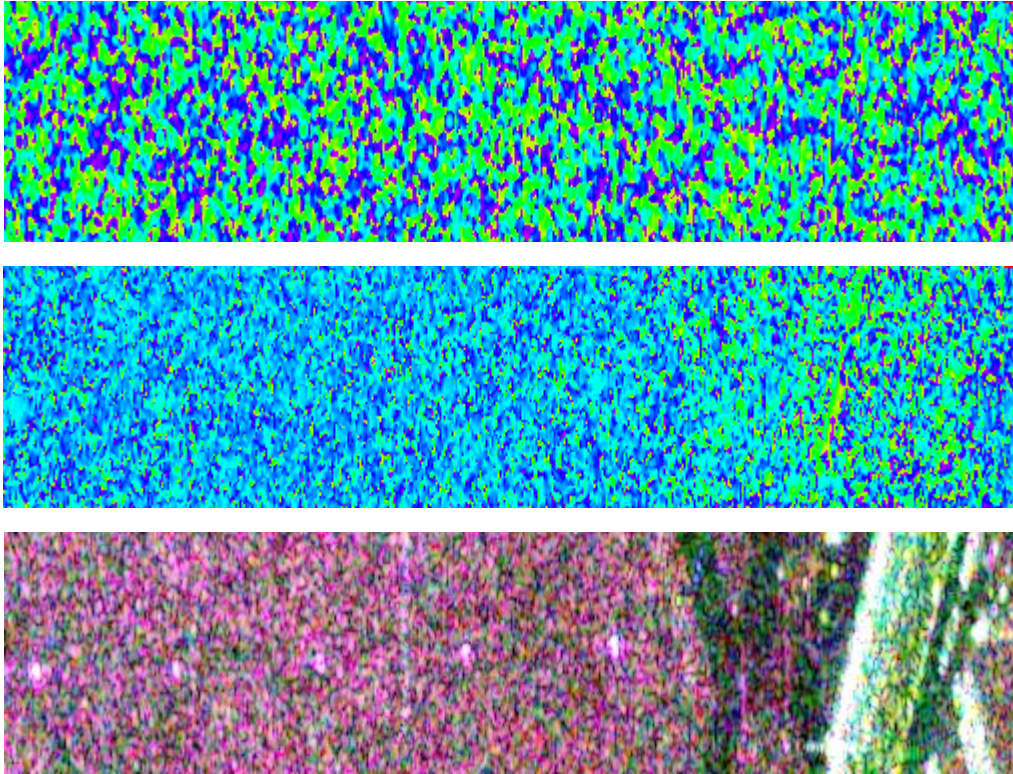
Fig. 4: \text{Arg}(S_{11}) (top) and \text{Arg}(S_{11}S_{22}^*) (middle) images.
