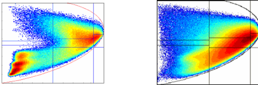
Fig. 7: Polarimetric data occurrence in the H-\alpha plane. San Francisco Bay (Left) and Oberpfaffenhofen (right).
