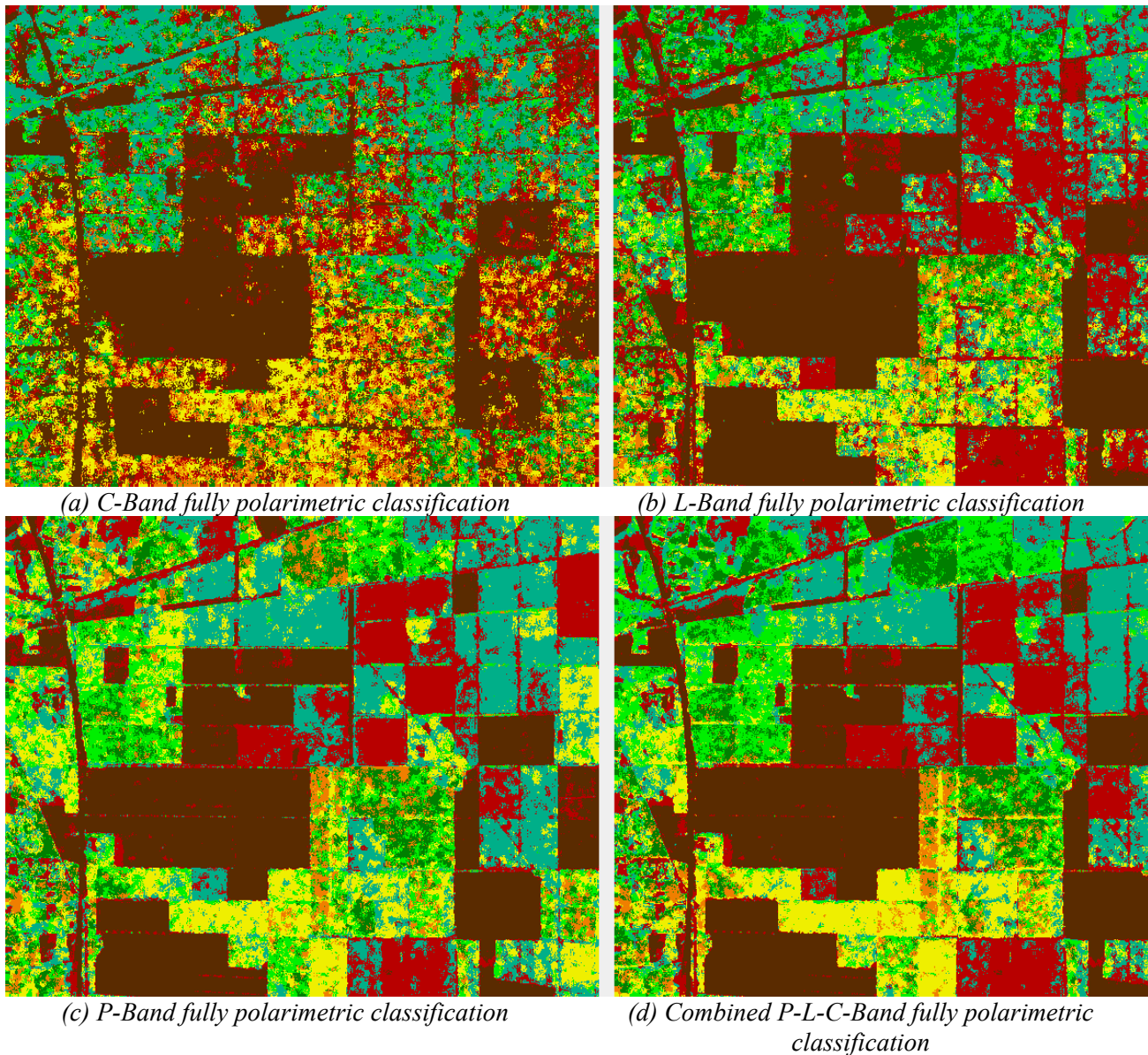
Fig. 5: Comparisons of fully polarimetric tree age classifications
