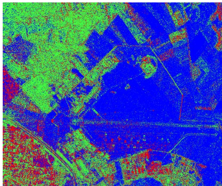
(b) Three scattering categories
