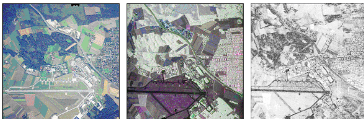
Fig. 14: Optical image (left), polarimetric color coded image (center) and interferometric coherence (right) over Oberpfaffenhofen (Germany)
