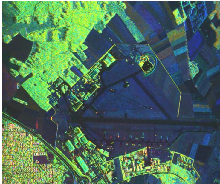
(a) Freeman decomposition
