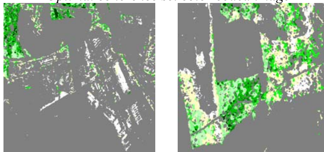
Volume diffusion classification results
