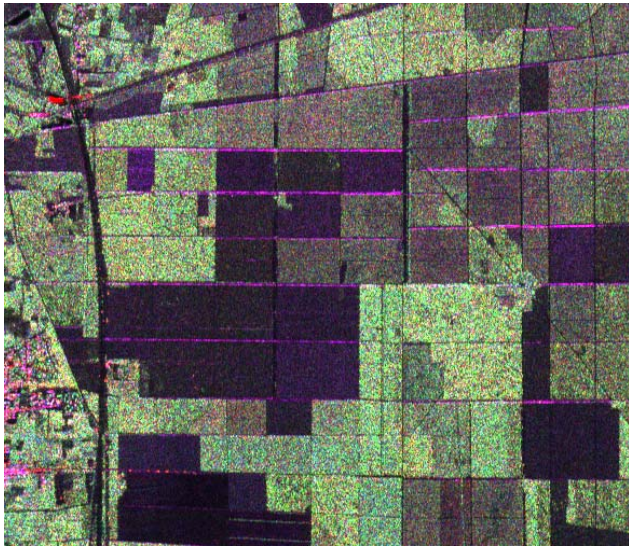
(a) P-band HH(Red), HV(Green) and VV(Blue)
