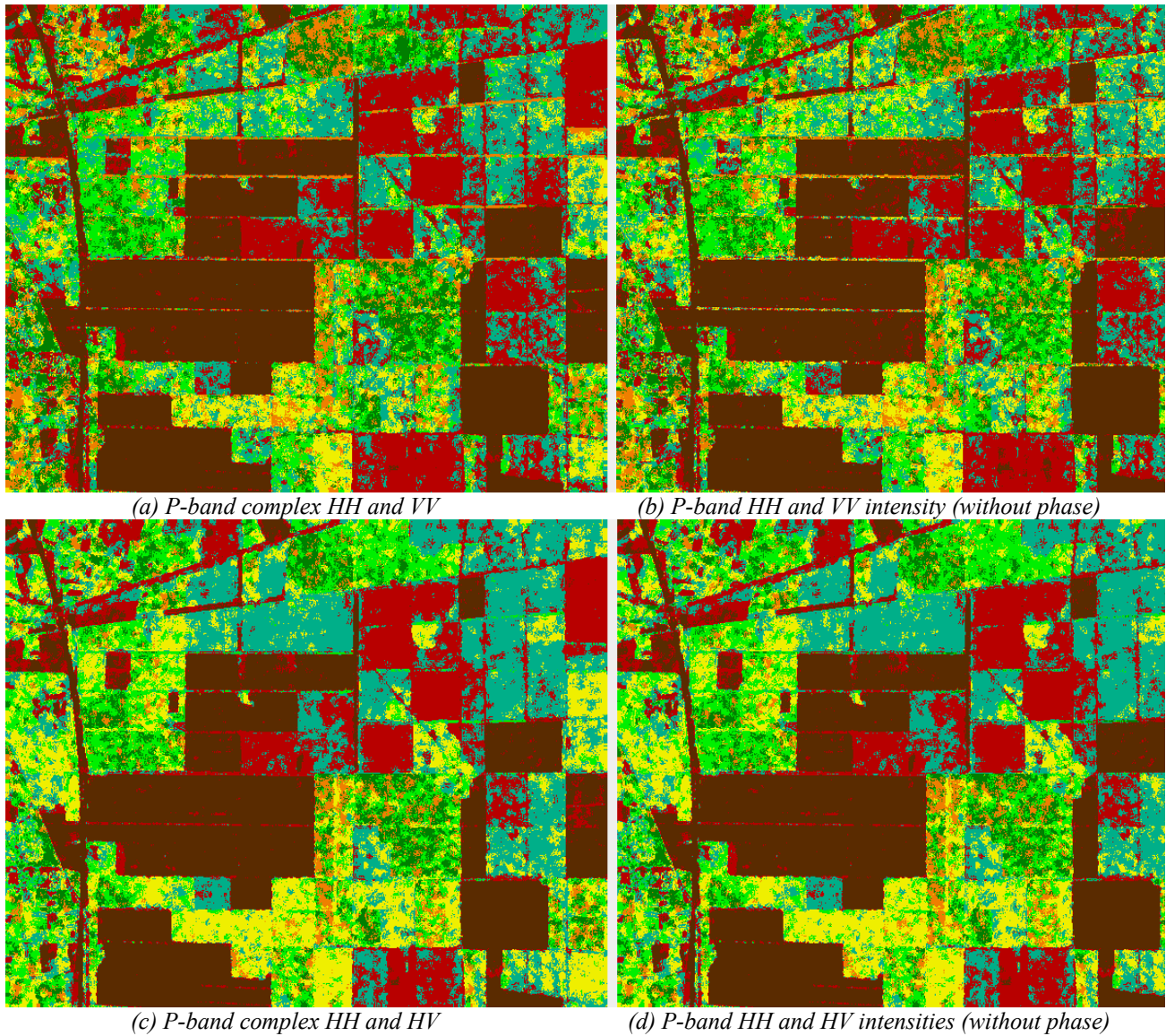
Fig. 6: Comparisons of dual polarization tree age classifications.
