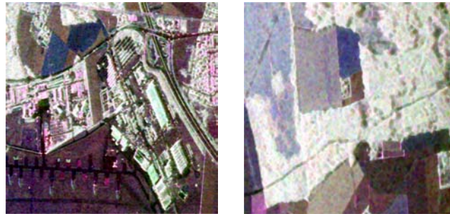
Polarimetric color coded image
