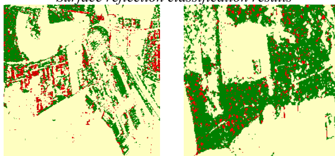
Classification into three canonical mechanisms including double bounce reflection
