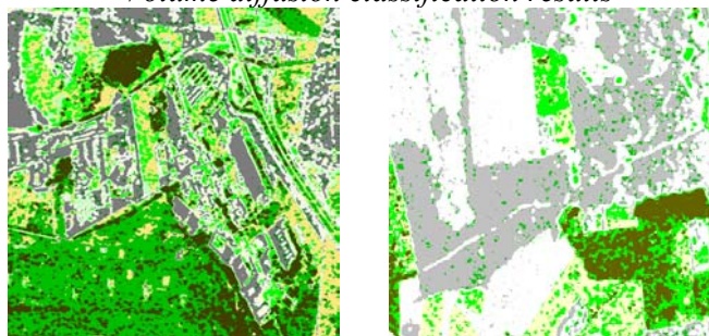
Surface reflection classification results
