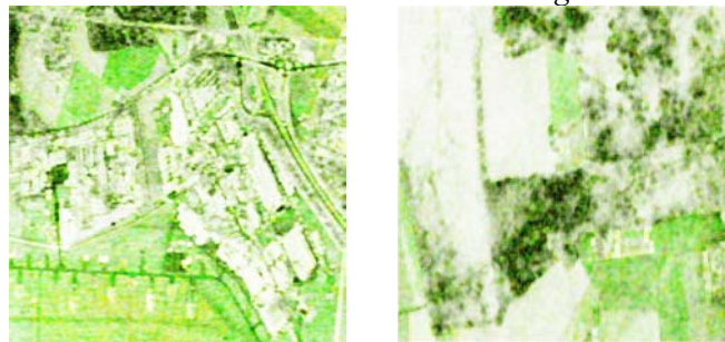
Optimal coherence set color coded image
