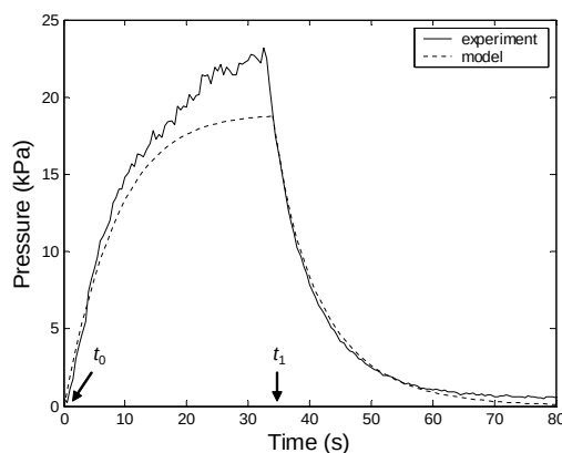
Figure 17: A trial in which a 0.2\ \mu\text{m} porous substrate without a BLM was pressurized by running the stepper motor at 5 Hz starting at time t_0 , and then turned off at time t_1 to allow pressure to decrease. The experimentally measured curve is marked by a solid line and the model based on a curve-fitted permeability is marked by a dotted line.
