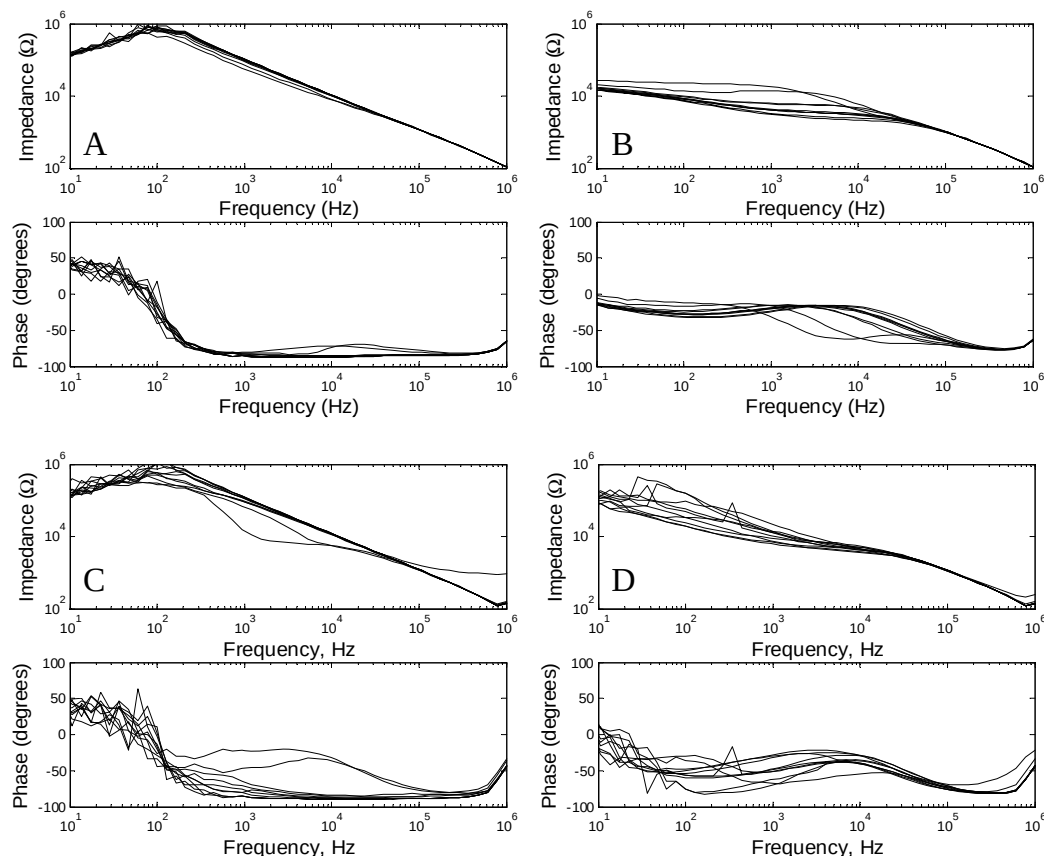
Figure 19: Impedance measurements (A) before pressurization of an SOPC BLM on a substrate with 0.2 \mu\text{m} diameter pores, (B) after pressurization of an SOPC BLM on a substrate with 0.2 \mu\text{m} diameter pores, (C) before pressurization of an SOPC BLM on a substrate with 2 \mu\text{m} diameter pores, and (D) after pressurization of an SOPC BLM on a substrate with 2 \mu\text{m} diameter pores.
