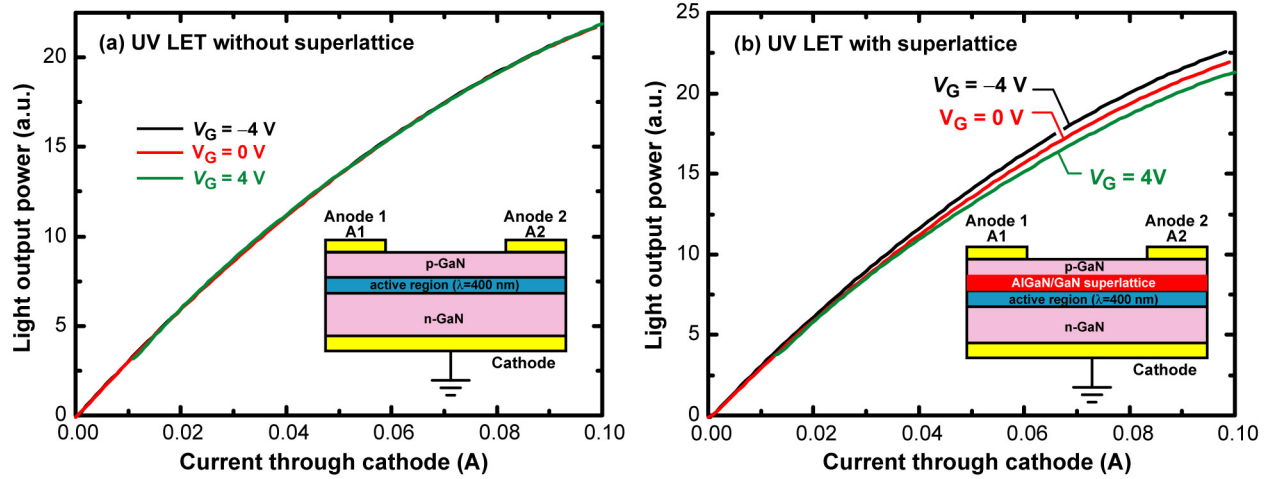
Figure 7: The light-output power-versus-current characteristic of the 400 nm UV LETs (a) without and (b) with AlGaIn/GaN SLs.
