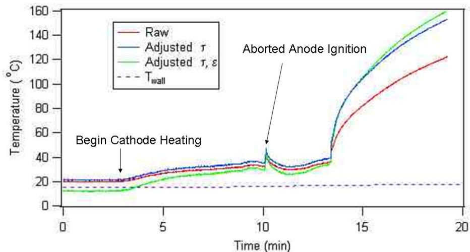
Figure 10. 600 W Thruster Inner Insulator Ring Temperature versus Time as seen from 90° with adjustments for measured viewport transmission and boron nitride emissivity
