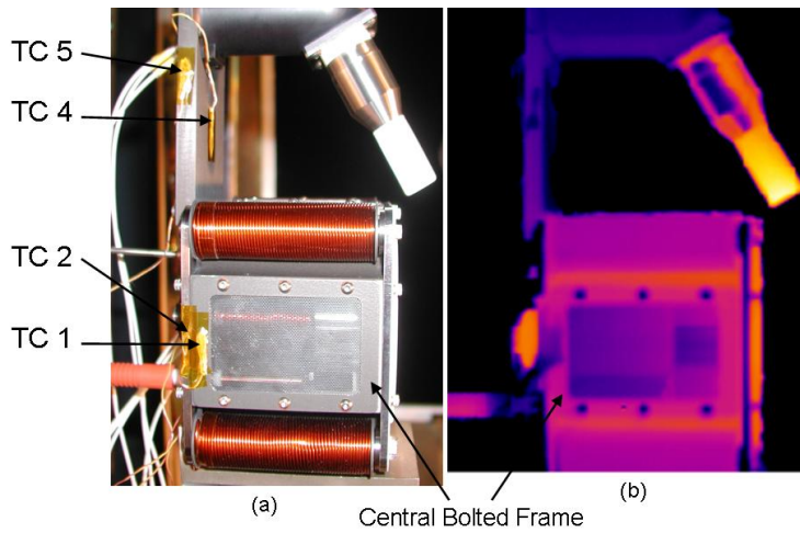
Figure 5. Busek BHT-600 Hall thruster installed on rotary stage (a) showing TC's (b) IR, firing at 0°
