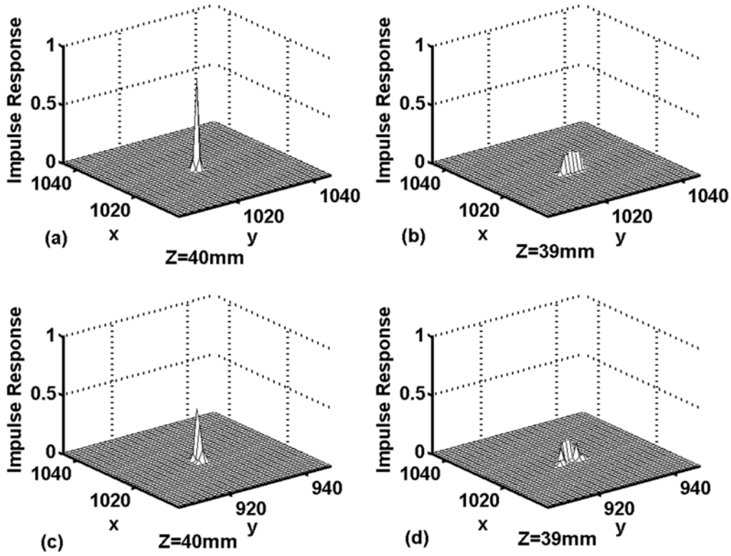
FIG. 5. Traditional SAA and point-by-point BP impulse responses: 25 projection images 480 and 25^\circ angular range, with the impulse located 40mm above the detector and about 4cm away from the chest wall. (a) and (b) give the impulse response of point-by-point BP; (c) and (d) give the impulse response of traditional SAA. (a) and (c) are impulse responses in the plane at the exact height of the impulse's location; (b) and (d) give corresponding values in a reconstruction plane 1 mm below the impulse's location.
