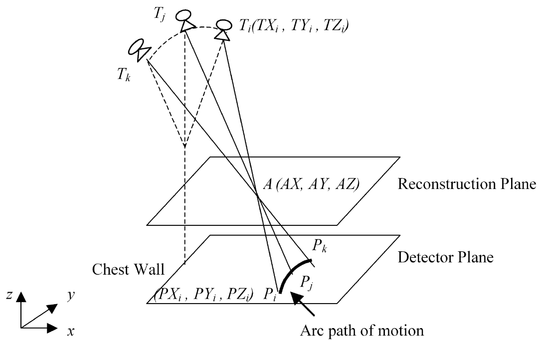
FIG. 2. Two-dimensional arc path from isocentric tube motion
