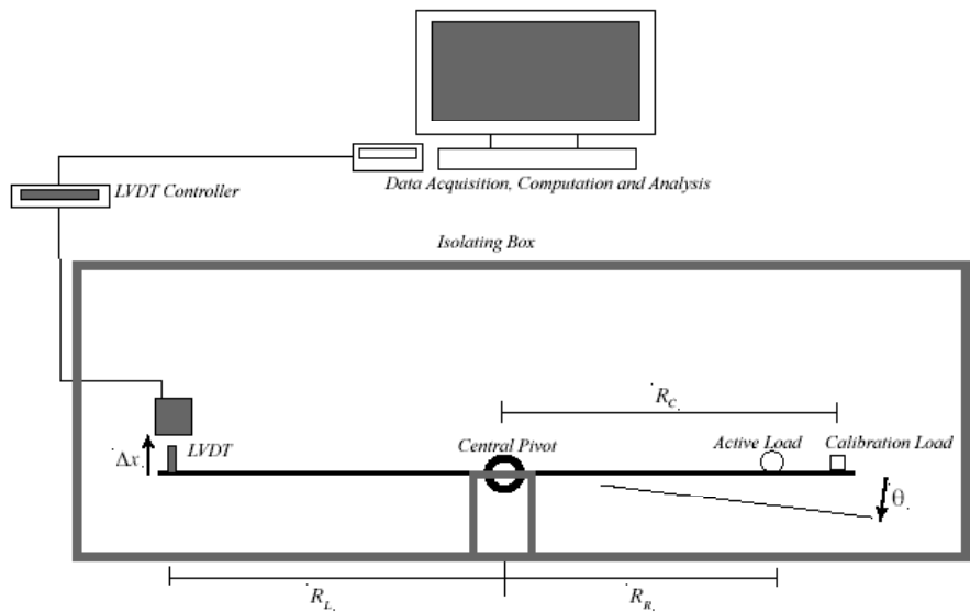
Figure 3. Schematic of the experimental setup
