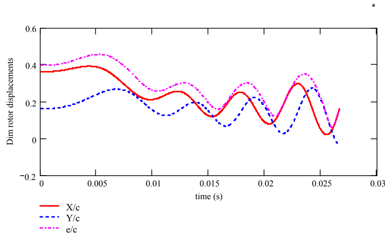
Figure 6b. Predicted dimensionless journal (rotor) eccentricity components versus time. Rotor mass M=10 kg
