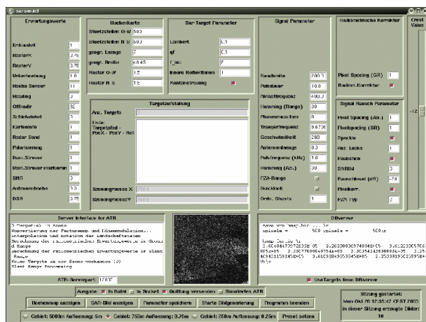
Figure 5 GUI of the SAR simulator
