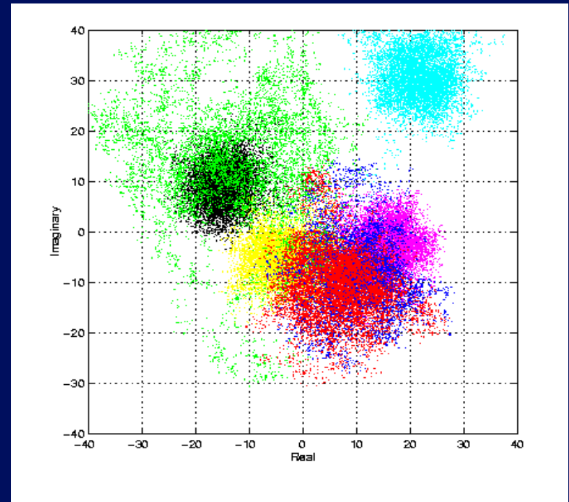
Scatterers 8-14
