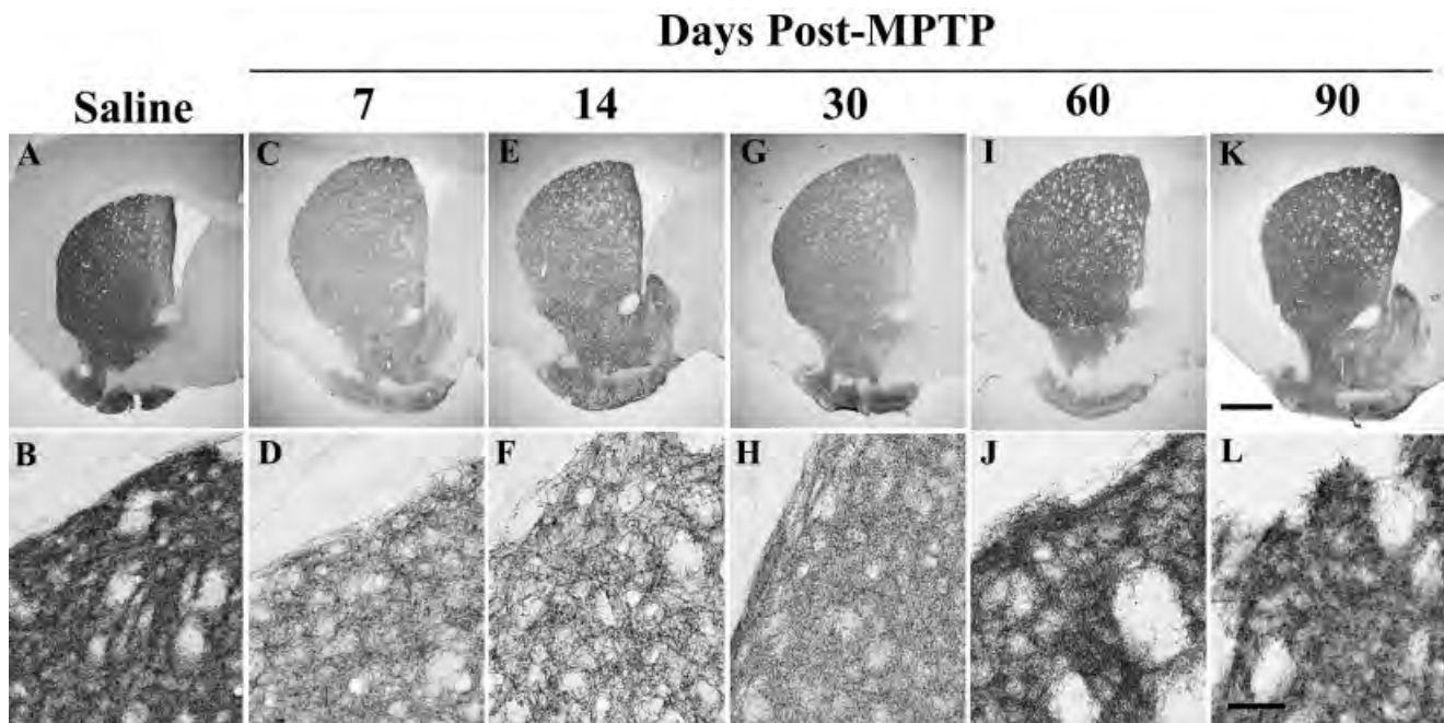
Fig. 7. Immunocytochemical analysis of DAT protein in the striatum after MPTP lesioning. Tissue sections in the coronal plane through the midbrain (Bregma 1.00) were stained with an antibody against the DAT protein. Images were made at low magnification (20 \times ; upper panels) to show an entire coronal hemisphere and at high magnification (400 \times ; upper panel) from the uppermost dorsal-lateral quadrant of the striatum apposing the corpus callosum). Saline-injected mice showed
