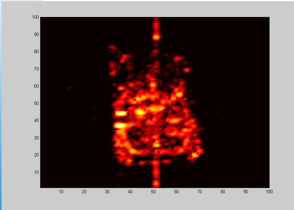
Threshold ISAR Image
