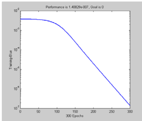
Output Error curve obtained during Training
