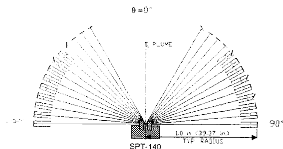
Fig. 5. Illustration of the placement of exposure samples with respect to the SPT-140.
