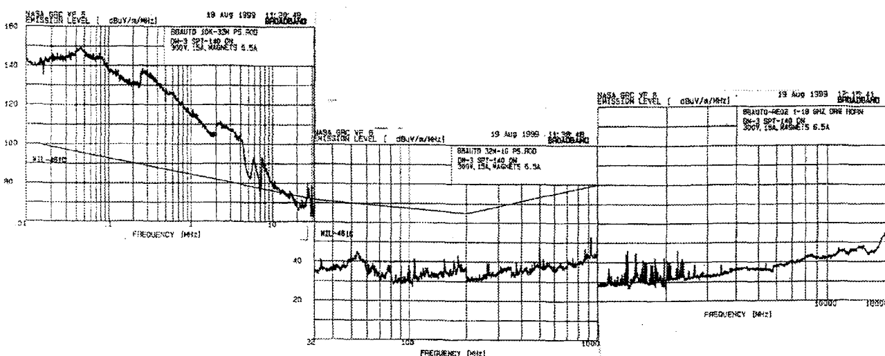
Fig. 9. E-field emissions for thruster firing at 4.5 kW. (Note horizontal scale change at breakpoints.)
