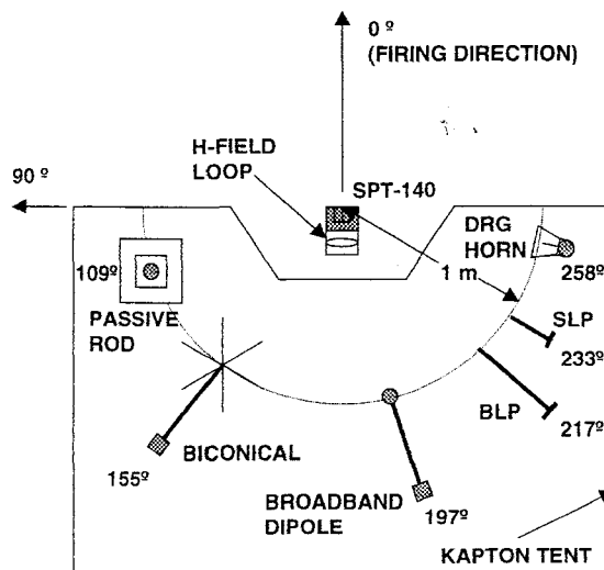
Fig. 7. Top view of EMI pallet.
