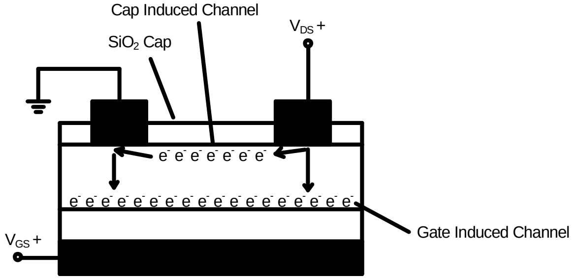
Figure 5.21: A schematic of an \text{SiO}_2 capped TTFT. The arrows indicate the direction of current flow and e^- indicates the presence of an electron channel.
