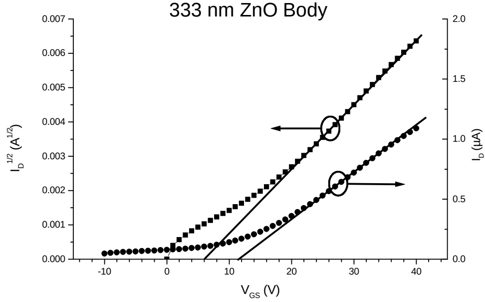
Figure 5.5: Linear region I_D - V_{GS} , V_{DS} = 0.5V , and saturation region I_D^{1/2} - V_{GS} , V_{DS} = V_{GS} , curves for an ion-beam sputtered ZnO TTFT with a body thickness of 333\text{ nm} on a NEG/ITO/ATO substrate. A linear extrapolation to I_D = 0 indicates a V_T of 6–12 V.
