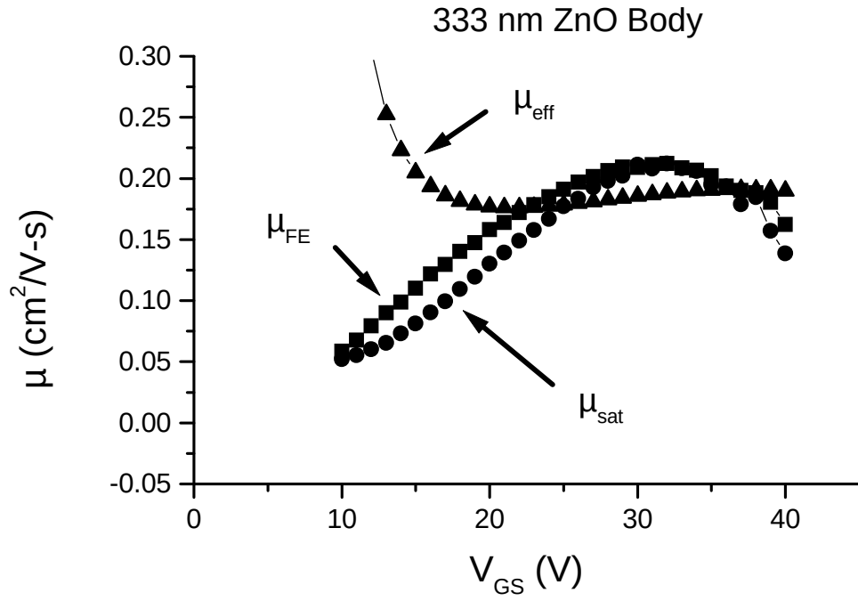
Figure 5.6: \mu_{sat} , \mu_{eff} , and \mu_{FE} versus V_{GS} curves for an ion-beam sputtered ZnO TTFT with a body thickness of 333\text{ nm} on a NEG/ITO/ATO substrate.
