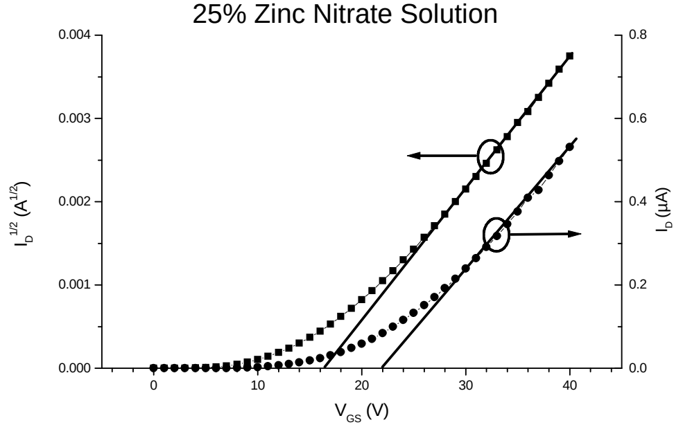
Figure 5.14: Linear region I_D - V_{GS} , V_{DS} = 0.5 V , and saturation region I_D^{1/2} - V_{GS} , V_{DS} = V_{GS} , curves for a spin-coated ZnO TTFT fabricated using 25% zinc nitrate spin solution with a body thickness of 32 nm on a NEG/ITO/ATO substrate. A linear extrapolation to I_D = 0 indicates a V_T of 16 V.
