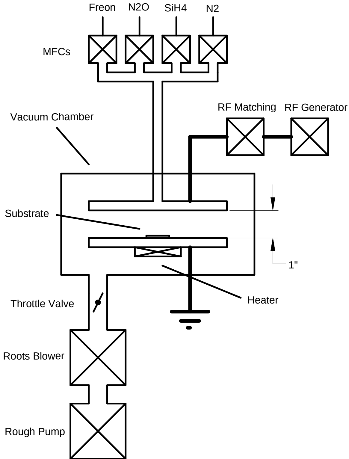
Figure B.1: A schematic of the PECVD system at Oregon State University.
