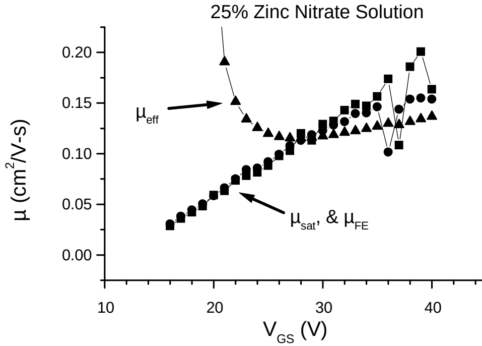
Figure 5.15: \mu_{sat} , \mu_{eff} , and \mu_{FE} versus V_{GS} curves for a spin-coated ZnO TTFT fabricated using 25% zinc nitrate spin solution with a body thickness of 32 nm on a NEG/ITO/ATO substrate.
