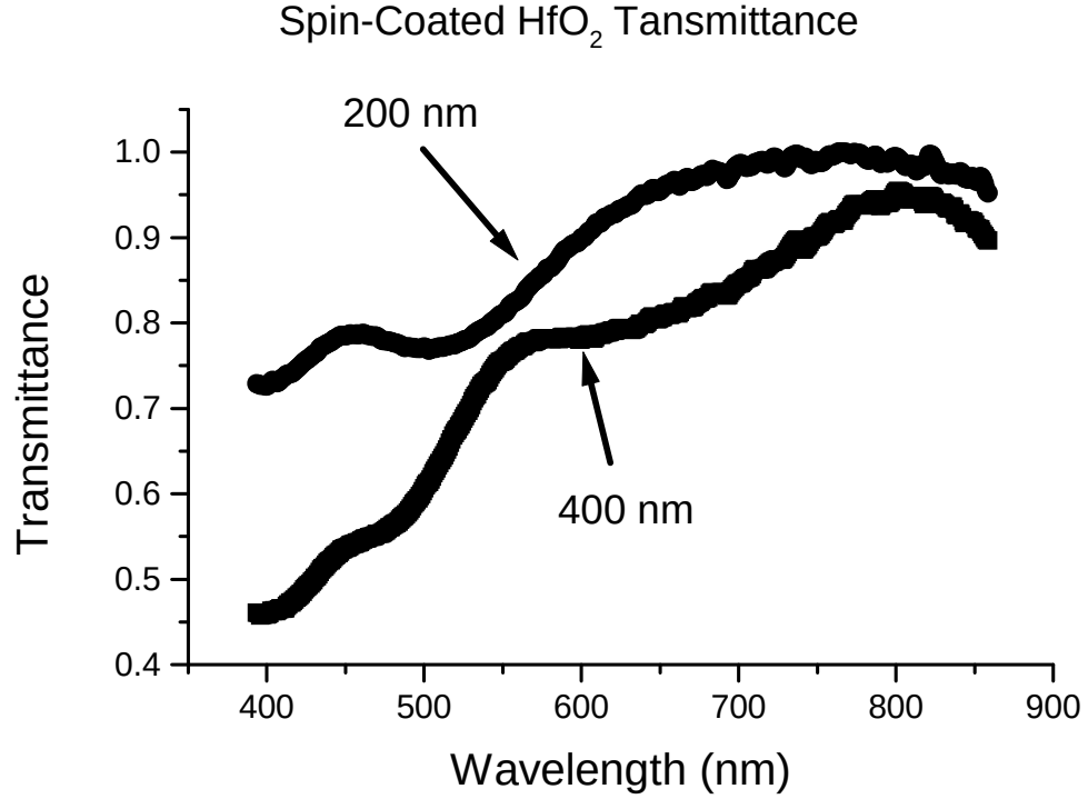
Figure 4.23: Transmittance versus wavelength curves for spin-coated HfO 2 with thickness of 200 and 400 nm. The substrate absorption curve has been subtracted out of these curves.
